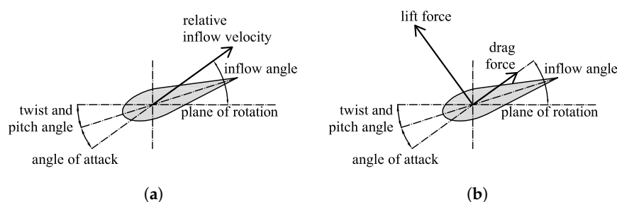
Figure 7. Schematic representation of (a) an aerofoil exposed to the relative inflow velocity resulting from the wind speed, the rotor speed and the structural motion, and (b) the resulting lift and drag forces acting on that aerofoil.
