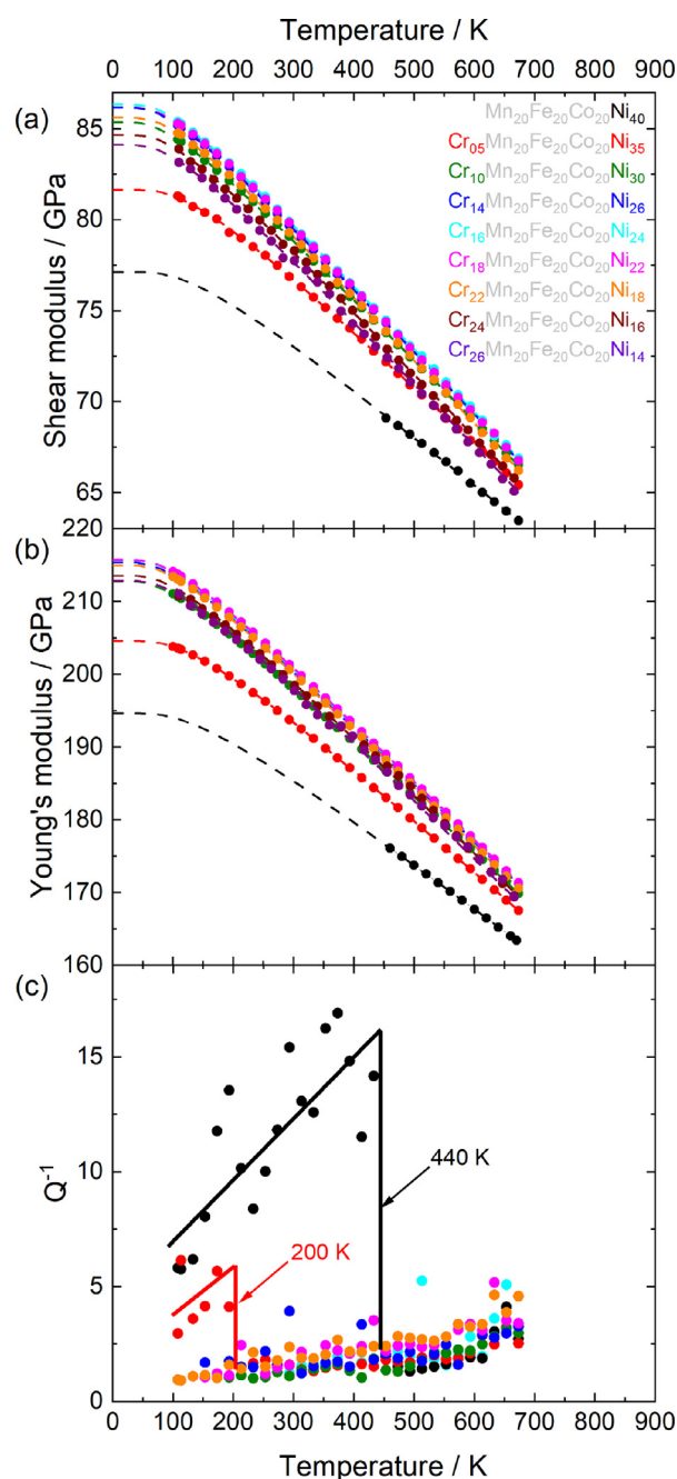
Fig. 5. Temperature dependence of elastic properties. (a) Shear modulus, (b) Young's modulus, and (c) inverse quality factor Q^{-1} of selected eigen modes. In (a) and (b), dots represent measured points, dashed lines are fits using Varshni's equation [39], see Eqs. S3, S4 and fitting parameters in Table 4.
