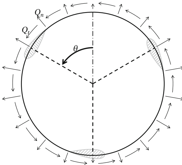
Fig. 8 Actuator cylinder model. (Adapted from De Tavernier 2021)
