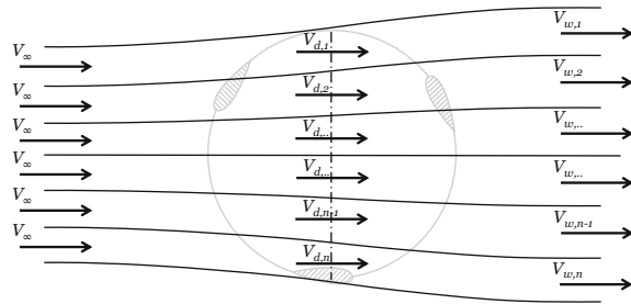
(b) Multiple-streamtube model
