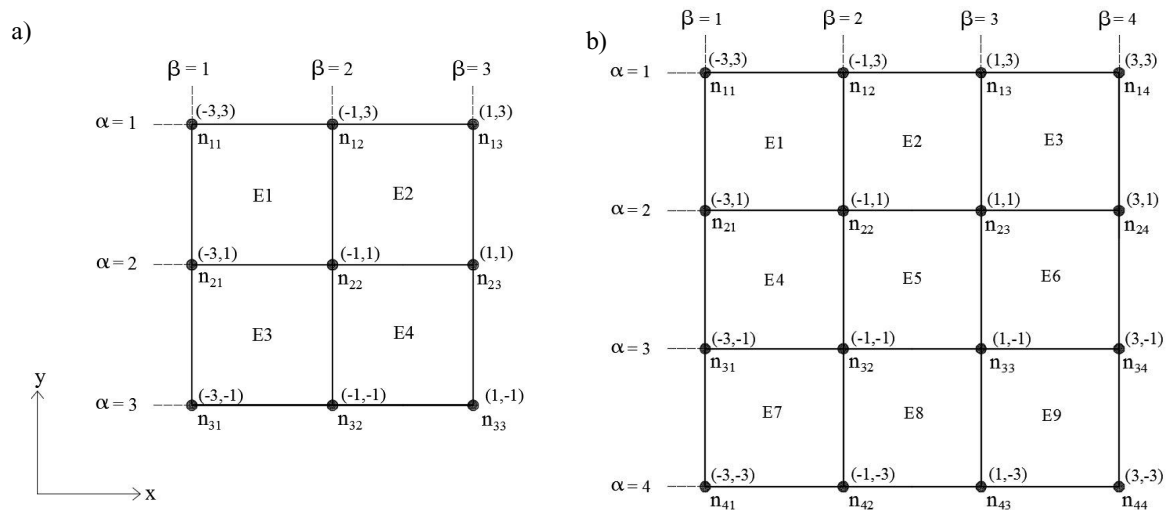
Fig. 4. Solution domain for C^I continuity for (a) boundary element E4 and (b) middle element E5.
