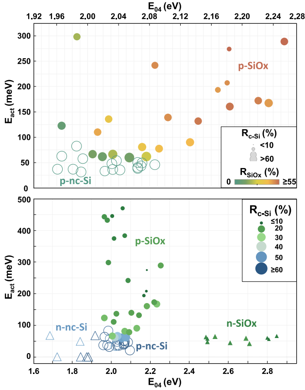
Fig. 6. E_{act} as a function of E_{04} for all doped a/nc-SiO x :H samples (bottom) and exclusively p-type a/nc-SiO x :H samples (top). nc-Si:H samples are represented by open symbols, while SiO x :H samples are represented by closed symbols. P-doped samples are represented by circles, while n-doped samples (bottom plot) are represented by triangles. In the top plot, the color and brightness of the symbols indicates R_{SiO_x} , while the size of the symbols indicates R_{c-Si} . In the bottom plot both symbol color/brightness and size indicate R_{c-Si} .
