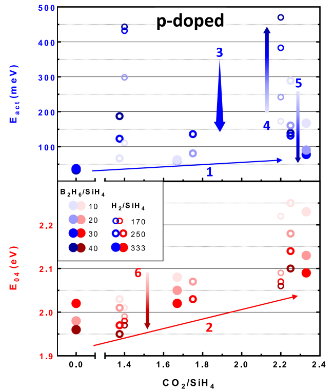
Fig. 3. E_{\text{act}} (top) and E_{04} (bottom) of p-doped a/nc-SiO x :H films as a function of the relative \text{CO}_2 flow rate ( F_{\text{CO}_2/\text{SiH}_4} ). The brightness/depth of color of the markers indicates the relative doping flow rate ( F_{\text{B}_2\text{H}_6/\text{SiH}_4} ) while the size of the markers and their open/closed nature indicates the relative hydrogen flow rate ( F_{\text{H}_2/\text{SiH}_4} ). Arrows, added to indicate trends in the data, are referenced in the article. ↑1–2 indicate the influence of F_{\text{CO}_2/\text{SiH}_4} . ↑3 indicates the influence of F_{\text{H}_2/\text{SiH}_4} . ↑4–6 indicate the influence of F_{\text{B}_2\text{H}_6/\text{SiH}_4} .
