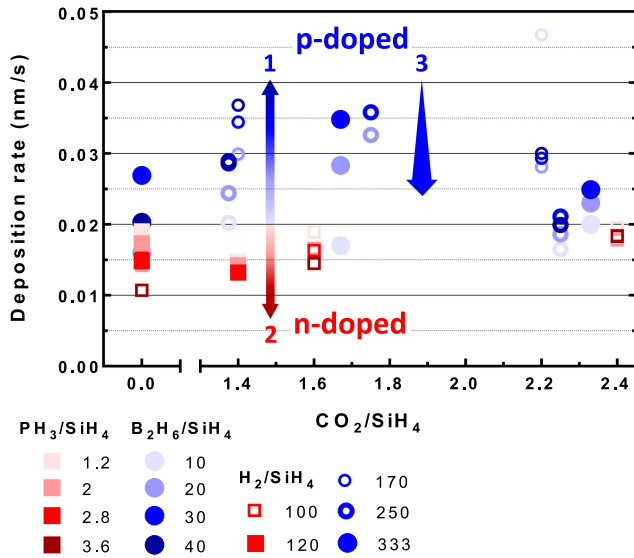
Fig. 5. Deposition rate of n-doped (red, squares) and p-doped (blue, circles) a/nC-SiO x>0 :H films, as a function of F_{CO_2/SiH_4} . The brightness/depth of color of the markers indicates the F_{PH_3/SiH_4} while the size of the markers and their open/closed nature indicates the F_{H_2/SiH_4} . Arrows, added to indicate trends in the data, are referenced in the article. ↑1-2 indicate the influence of F_{B_2H_6/SiH_4} and F_{PH_3/SiH_4} . ↑3 indicates the influence of F_{H_2/SiH_4} .
