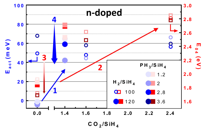
Fig. 4. E_{\text{act}} (left, circles) and E_{04} (right, squares) n-doped a/nc-SiO x :H films as a function of F_{\text{CO}_2/\text{SiH}_4} . The brightness/depth of color of the markers indicates the F_{\text{PH}_3/\text{SiH}_4} while the size of the markers and their open/closed nature indicates F_{\text{H}_2/\text{SiH}_4} . Arrows, added to indicate trends in the data, are referenced in the article. ↑1–2 indicate the influence of F_{\text{CO}_2/\text{SiH}_4} . ↑3 indicates the influence of F_{\text{PH}_3/\text{SiH}_4} . ↑4 indicates the influence of F_{\text{H}_2/\text{SiH}_4} .
