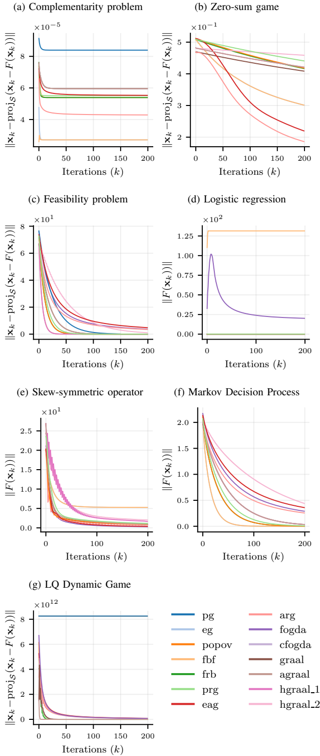
Fig. 1. Convergence results for each example, using the currently available algorithms in monviso .
