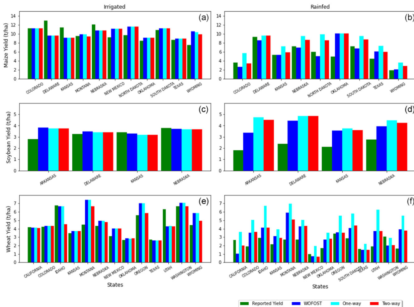
Figure 5. Spatial (i.e., state-level) analysis of irrigated and rainfed crops of (a, b) maize, (c, d) soybean, and (e, f) wheat for the years 2006 to 2019 for the CONUS region.
