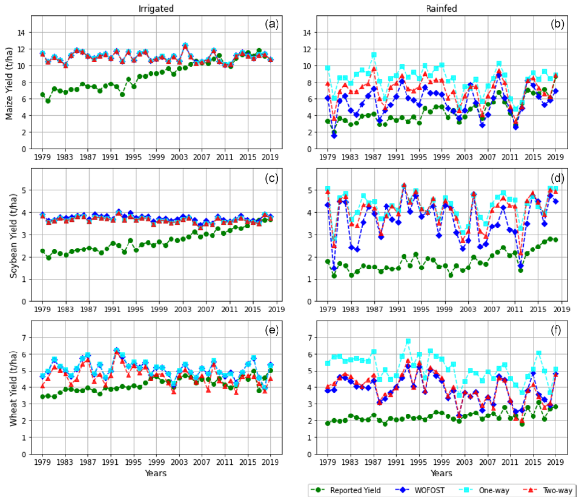
Figure 4. Temporal analysis of irrigated and rainfed crops of (a, b) maize, (c, d) soybean, and (e, f) wheat for the years 1979 to 2019 for the CONUS region.
