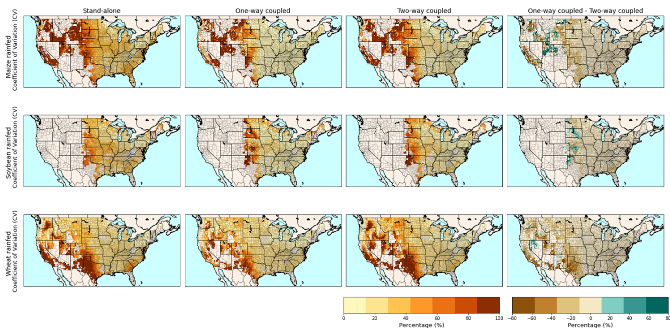
Figure 9. Coefficient of variation (CV) over 1979–2019 of rainfed crop yields for maize, soybean, and wheat within CONUS as obtained under stand-alone, one-way, and two-way coupling and the difference between one-way and two-way coupling.
