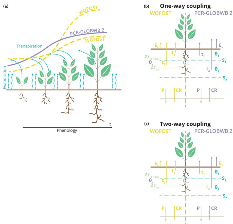
Figure 3. Schematic view of the coupled model framework: panel (a) shows the calculated phenology from WOFOST and PCR-GLOBWB 2 over time along with the associated fluxes. Panel (b) displays a detailed representation of the one-way coupling approach, where soil moisture is transferred from PCR-GLOBWB 2 to WOFOST, and panel (c) illustrates the two-way coupling approach, where variables are exchanged in both directions between PCR-GLOBWB 2 and WOFOST.
