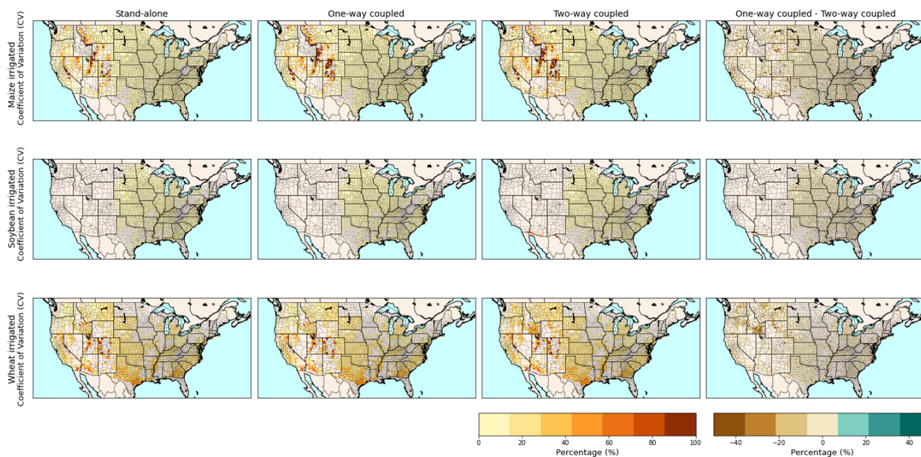
Figure 8. Coefficient of variation (CV) over 1979–2019 of irrigated crop yields for maize, soybean, and wheat within CONUS as obtained under stand-alone, one-way, and two-way coupling and the difference between one-way and two-way coupling.
