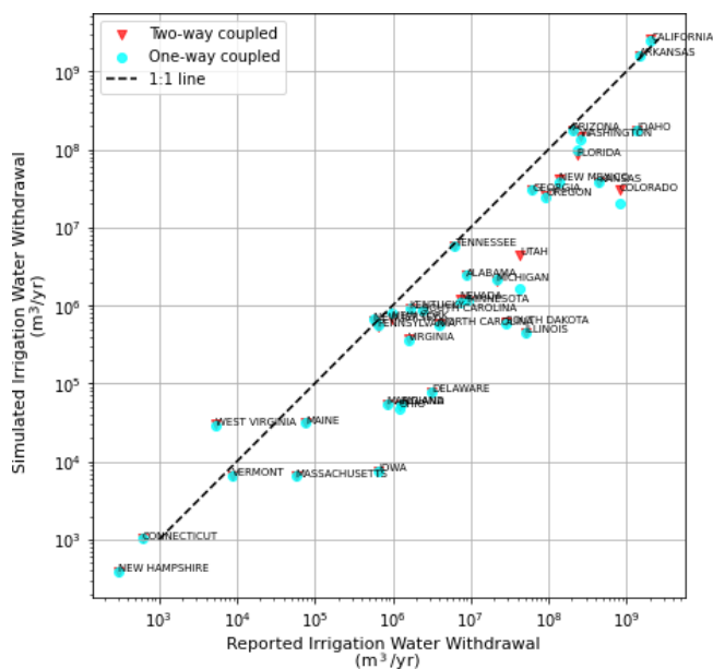
Figure 10. Spatial variation of one-way and two-way irrigation water withdrawal compared with USGS-reported water withdrawal data per state for all crops across the CONUS region with a logarithmic scale.
