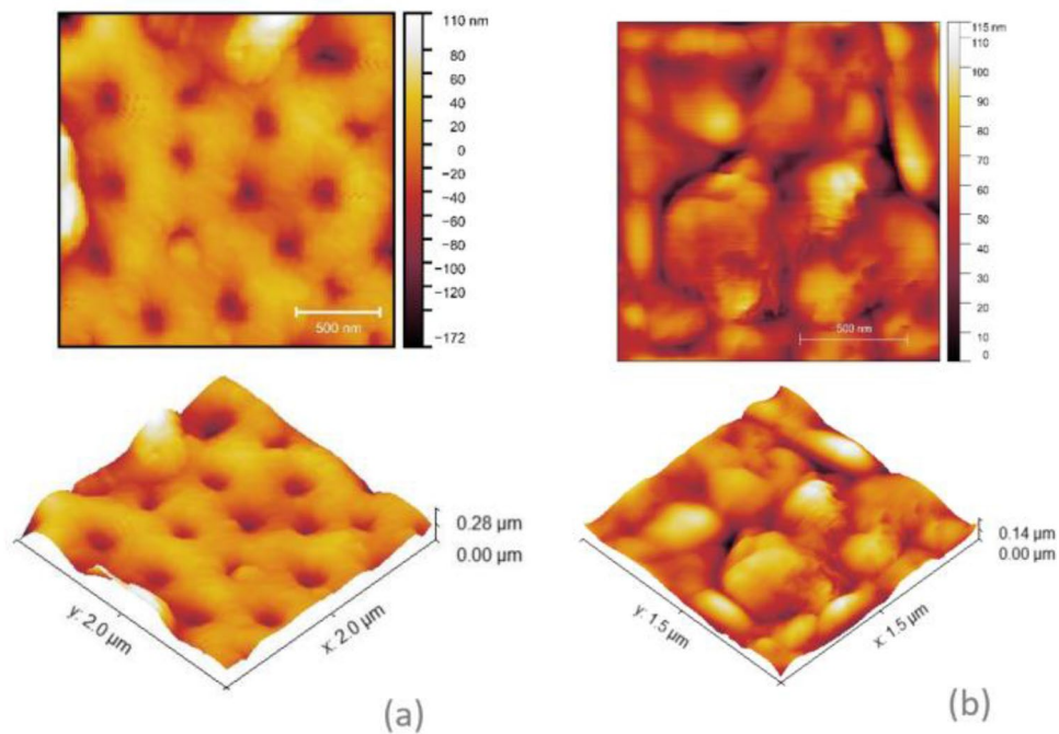
Fig. 6 AFM scans of a pristine and b Highly lithiated flake surface
