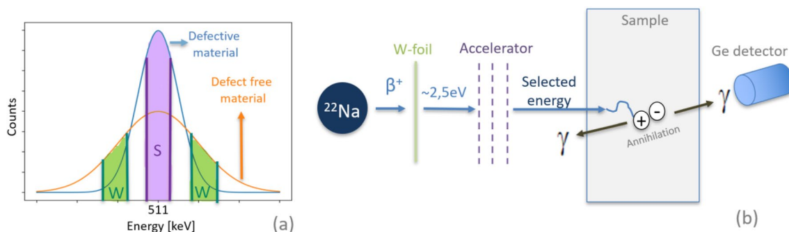
Fig. 2 a Energy distribution spectra of a defect-free sample (orange) and a defective material (blue), and the shape parameters S (purple) and W (green). b PADBS measurement principle for single-detector mode in which one out of the two Gamma rays is detected
