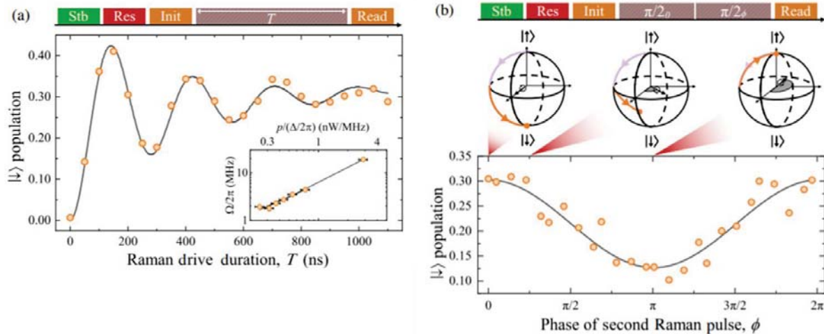
FIG. 1. Multiaxis coherent spin-qubit control. (a) |\downarrow\rangle population (orange circles) as a function of the Raman drive duration T with the pulse sequence shown at the top. The Raman drive is applied with \Delta/2\pi = 1.2 GHz and p = 650(70) nW. The black curve is a fit to a two-level model under a master-equation. Inset: \Omega/2\pi as a function of p/(\Delta/2\pi) with a linear fit to the data (solid curve). Here, \Delta/2\pi and p are varied from 300 to 1200 MHz and 40 to 650 nW, respectively. (b) Pulse sequence (top) with one \pi/2 pulse about x and a second about an axis rotated by an azimuthal angle \phi from the x axis. The \pi/2 pulse duration is determined from Rabi measurements taken with \Delta/2\pi = 300 MHz and p = 260(30) nW. Illustrated on the Bloch spheres are trajectories for \phi = 0 (left), \phi = \pi/4 (center), and \phi = \pi (right). The |\downarrow\rangle population (orange circles) is plotted as a function of \phi . The solid curve is a cosine function.
