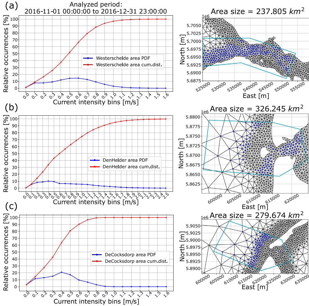
Fig. 10. Intensities PDF computed at different areas: (a) Westerschelde, (b) Den Helder, (c) De Cocksdorp. Mesh nodes in blue have an estimated depth > 10 m with respect to MSL. Relative occurrences normalized by the total amount of analyzed data with the contribution of all nodes in blue. Intensities bin width is 0.1 \text{ ms}^{-1} . The area size corresponds to the one defined by the polygon in cyan. Offshore extension of polygons for (b) and (c) is \sim 20 km.
