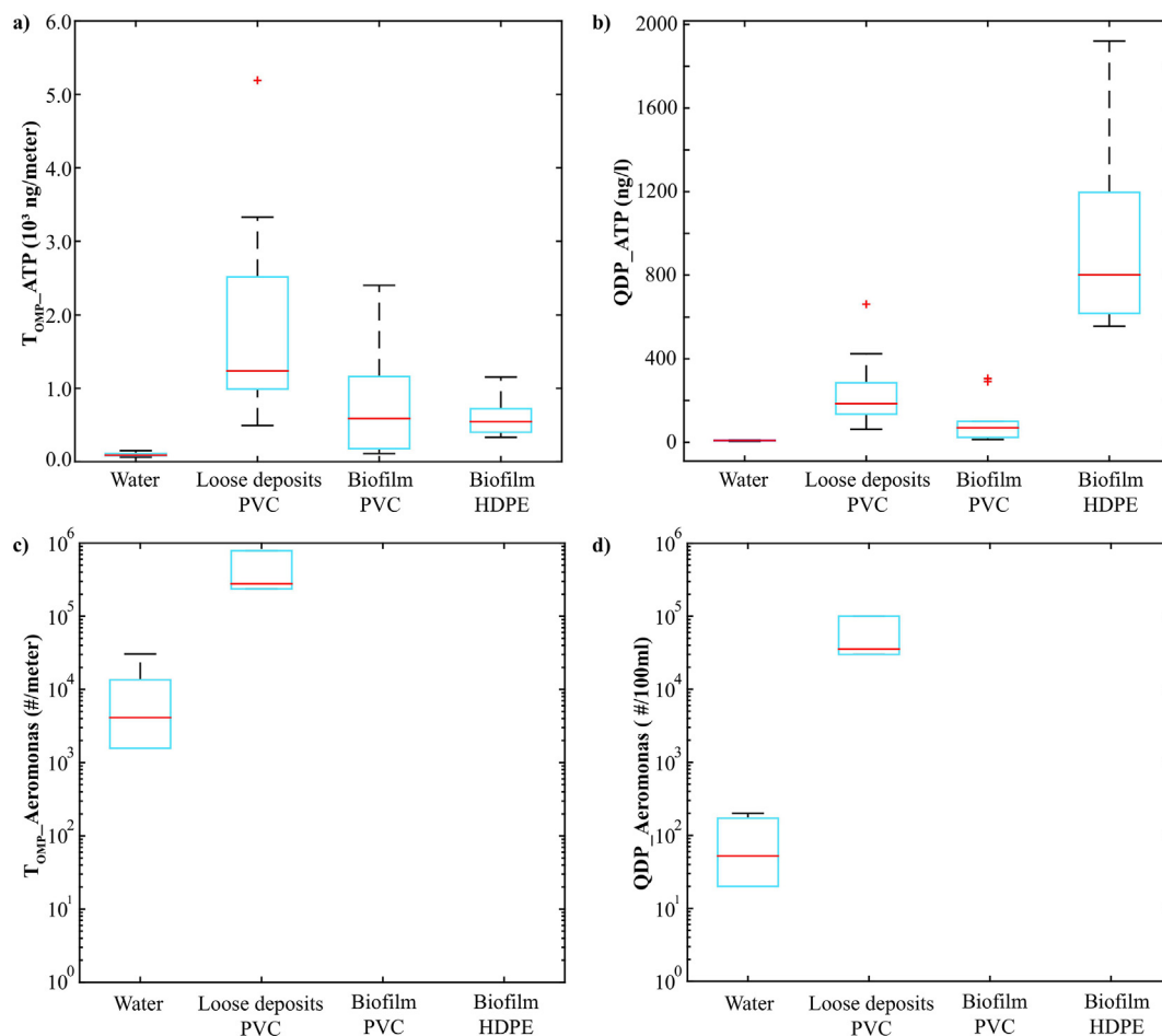
Fig. 3. Boxplot showing the distribution of active biomass (ATP and Aeromonas ) across niches normalized back to 1 m of pipe ( n = 10 ); the values obtained from water samples are included to provide an indication of the relative values in loose deposits, PVC-U biofilm, and HDPE biofilm.
