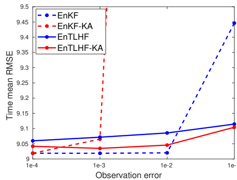
Figure 6.2: Error evaluation of the robust and non-robust methods respect to the observation error.
