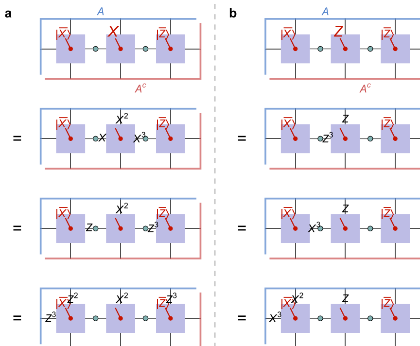
Fig. 7 | Graphical proof of the state-dependent reconstruction of the central ququart in Fig. 5c. a The ququart Pauli operator \bar{X} is represented by the logical operator \bar{X} = X X^2 X^3 I . After pushing the Pauli operators acting on internal indices through the B tensors (green dots), which exchanges X \leftrightarrow Z , we apply the stabilizer
