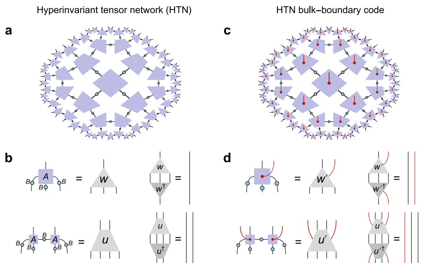
Fig. 4 | Construction of a hyperinvariant tensor network (HTN) code. a The original HTN construction from Ref. 22,23 for a \{5, 4\} hyperbolic map; vertices and edges are associated with A and B tensors, respectively. b The isometry constraints for one- and two-vertex combinations of A and B . With these constraints, each radial layer of tensors acts isometrically, in the manner of an RG transformation.
