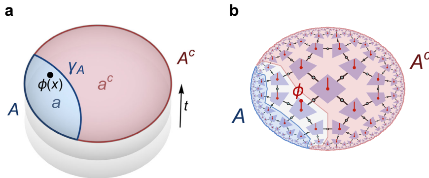
Fig. 1 | Complementary recovery in holography. a In continuum AdS/CFT on slices at constant time t , a bipartition of the boundary CFT into two regions A and A^c is equivalent to a bipartition of the bulk into two entanglement wedges a and a^c , separated by a Ryu-Takayanagi surface \gamma_A . Any bulk (field) operator \phi(x) can be
