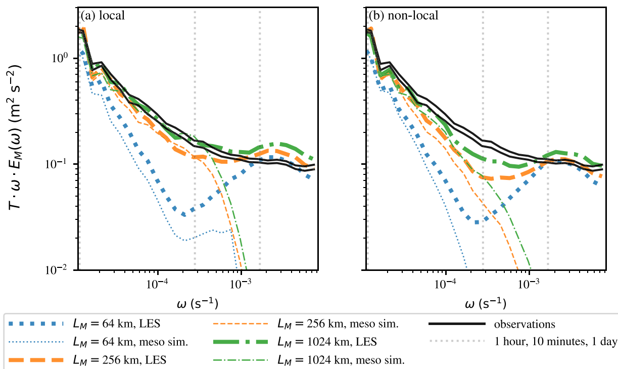
FIGURE 4 Spectra of the 80-m wind speed during 2022 for the different mesoscale domain sizes (indicated by different lines, thick lines for the LES, thin for the mesoscale simulations), with (a) local diffusion and (b) non-local diffusion. The LES domain size is 12.8 km.
