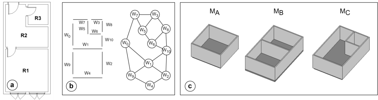
Figure 3. The illustrative example: a) the floor plan, b) the segment walls and their graph model, and c) the three topologies of VM units
