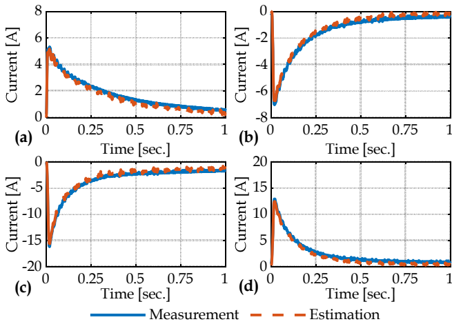
Fig. 12. Comparison between the DC component of the neutral current obtained from measurement and the of the three winding estimated DC components of the field testbed transformer: (a) Avg. Error =0.2055 [A]; (b) Avg. Error =0.23 [A]; (c) Avg. Error =0.4143 [A]; (d) Avg. Error =0.45 [A].
