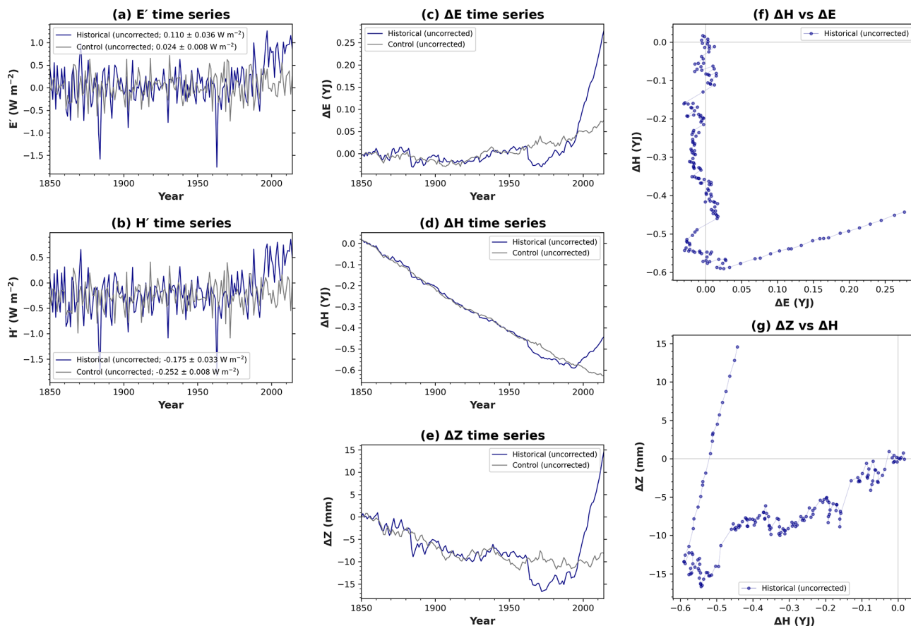
Figure 1. Uncorrected time series and bivariate relationships for the UK Earth System Model (UKESM1). These uncorrected time series have not yet been corrected for drift. Using data from the control and historical simulations, time series are shown for the following global variables: (a) top-of-atmosphere radiative flux ( E' ), (b) sea surface heat flux ( H' ), (c) excess system energy ( \Delta E ), (d) excess ocean heat ( \Delta H ), and (e) thermosteric sea level rise ( \Delta Z ). Global total E' and H' are expressed in global mean units of watts per square metre ( \text{W m}^{-2} ). In (a) and (b), the legend shows the mean of the entire time series and the standard error of the mean. In (a–e), only the segment of the control time series that corresponds to the historical period (1850–2014) is shown. (The full length of the entire control time series is 1100 years.) For the historical simulation, bivariate relationships are also shown: (f) \Delta H versus \Delta E and (g) \Delta Z versus \Delta H . Interpretation is offered in Sect. 4.1.
