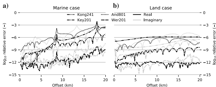
Figure 6. (a) The canonical marine CSEM model of Key (2012) and (b) a land model with the source and receiver at the surface. The new filter shows relative errors that are generally several orders of magnitude lower than for the other filters.
