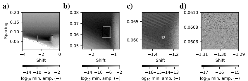
Figure 3. Solution spaces of four consecutive inversion runs for a 201 pt filter. Each consecutive run magnifies into a portion of the previous solution space, indicated by the square. The more in detail we obtain the solution space, the more random the distribution appears to be.
