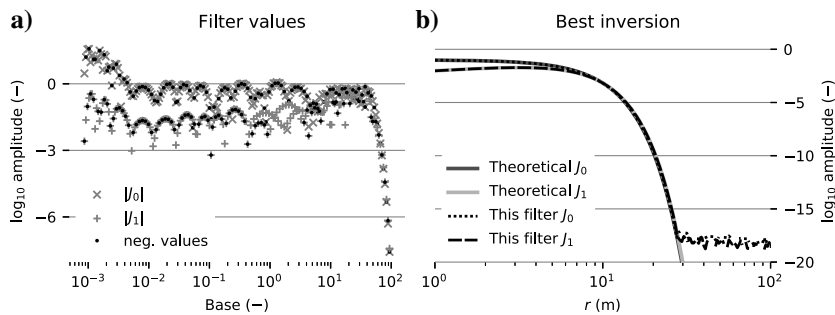
Figure 4. (a) Filter values of the best obtained 201 pt filter with the corresponding check of quality in (b). The black points indicate negative values, which show that adjacent values have often opposite signs.
