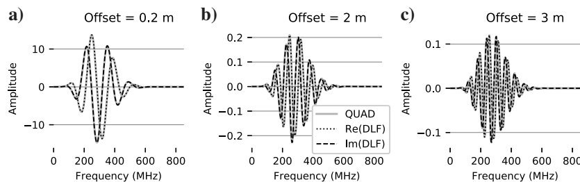
Figure 11. The real and imaginary parts of the frequency-domain response for the model given in Figure 9a with swapped first and second layers for horizontal offsets of (a) 0.2 m, (b) 2.0 m, and (c) 3.0 m.
