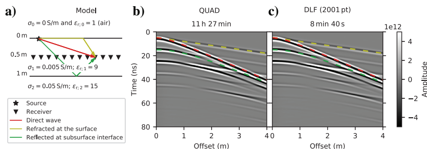
Figure 9. The GPR example for the model given in (a) using empymod with (b) adaptive quadrature (QUAD) or with (c) a 2001 pt DLF. QUAD took approximately 11 h 27 min to calculate, whereas DLF took 2 min 10 s in parallel on four nodes, hence under 9 min in total.
