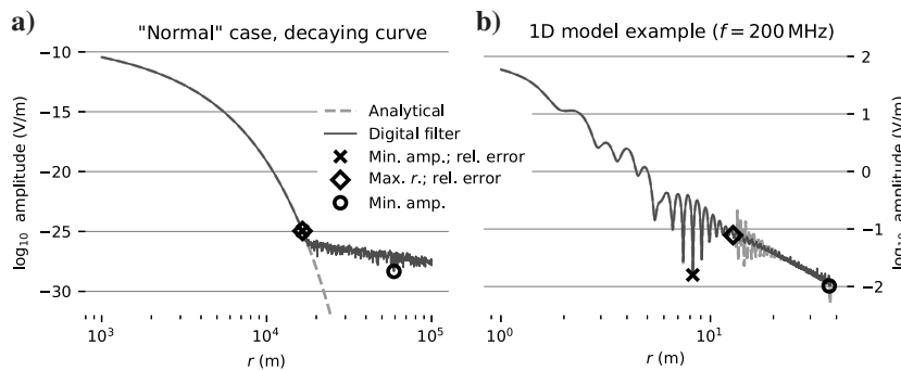
Figure 1. (a) A regular RHS curve of a transform pair with a purely decaying function. The minimum amplitude or maximum r yield the same result in this scenario. Using a relative error criteria is more stable than just the absolute minimum amplitude. (b) A 1D model for f = 200 MHz. Here, the maximum r provides better criteria for the inversion.
