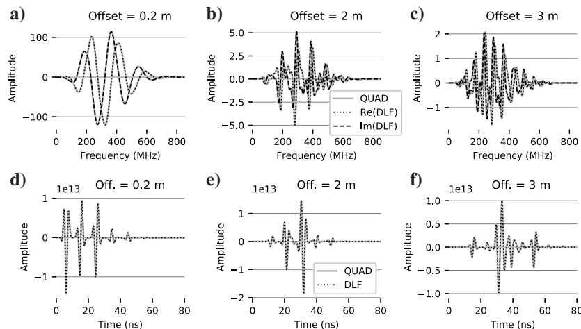
Figure 10. (a-c) The real and imaginary parts of the frequency-domain responses and (d-f) the time-domain responses for horizontal offsets of (a and d) 0.2 m, (b and e) 2.0 m, and (c and f) 3.0 m.
