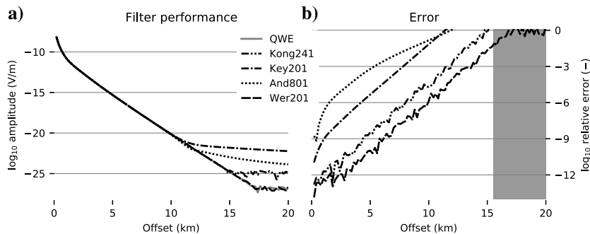
Figure 5. (a) Results of different filters and QWE for the model of Figure 5 from Kong (2007) with the relative errors shown in (b), using the QWE result. The relative error is meaningless from approximately 15.5 km onward because QWE failed as well for these very low amplitudes.
