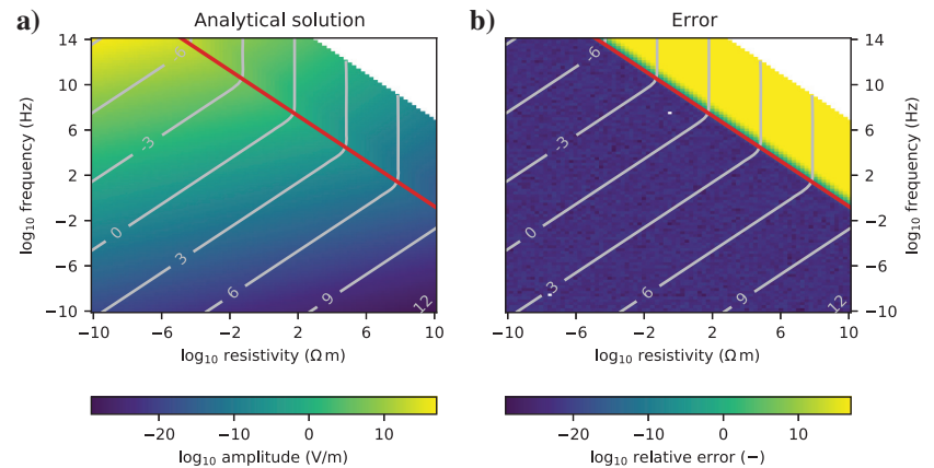
Figure 8. (a) Amplitude of the analytical full-space solution for a wide range of resistivities and frequencies. The contour lines show the \log_{10} scaled offset used for the calculation, where the offset is set to the skin depth. (b) Relative error of the DLF compared with the analytical solution. The filter Wer201 works well in the diffusive limit, but fails when wave phenomena become dominant. The red line shows where \omega \epsilon \rho = 1 .
