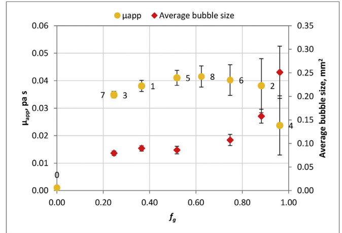
Fig. 13. Foam apparent viscosity \mu_{app} and average bubble size over a range of foam qualities; u_t = 0.0021 m/s. Error bars in \mu_{app} reflect fluctuations in pressure gradient. Error bars in bubble size indicate standard deviation in the bubble size.
