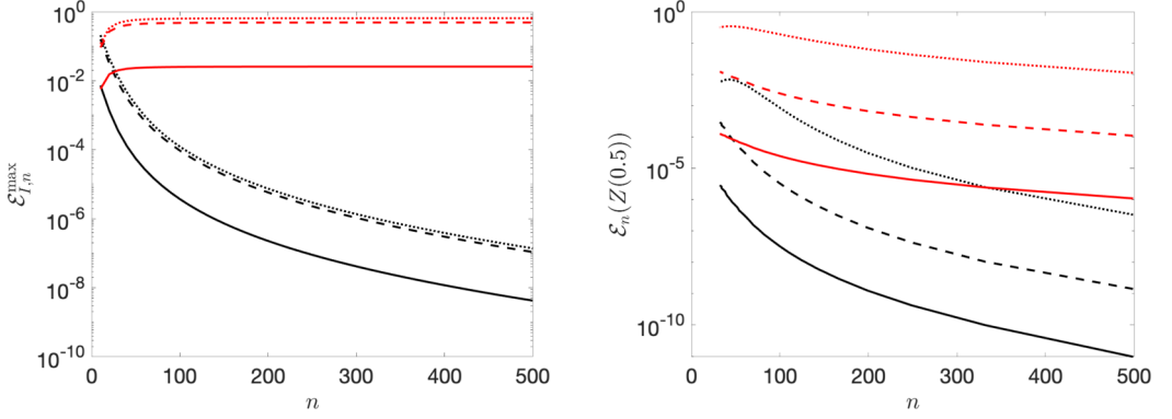
Figure 1. The results for model 1 (black) and model 2 (red) for the first example (5.2) with integral observations (left) and point observations (right). Solid lines correspond to \delta = 1 , dashed to \delta = 10 , and dotted to \delta = 100 .
