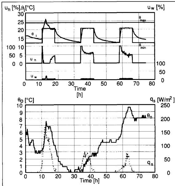
Fig. 4. Indoor temperature control. Heating situation.
