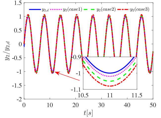
Fig. 5. Output y_2 under three cases.
