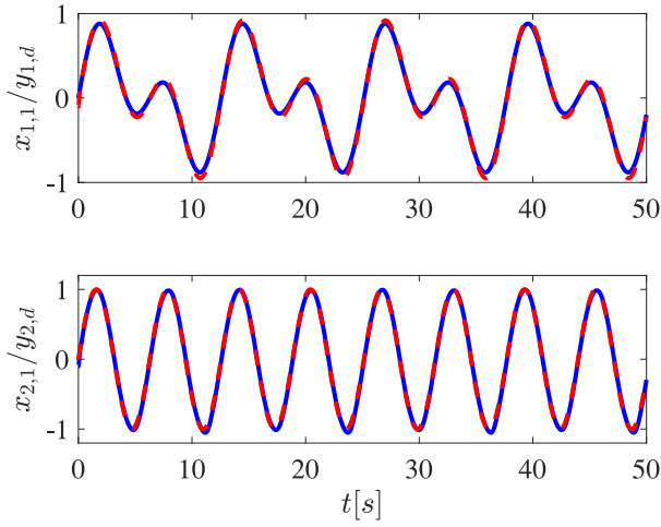
Fig. 1. Outputs y_1(x_{1,1}) and y_2(x_{2,1}) (dashed), and desired trajectories y_{1,d} and y_{2,d} (solid).
