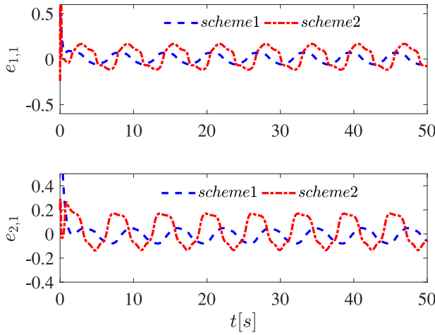
Fig. 9. Tracking errors of two schemes.
