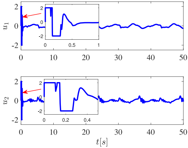
Fig. 2. System inputs u_1 and u_2 .
