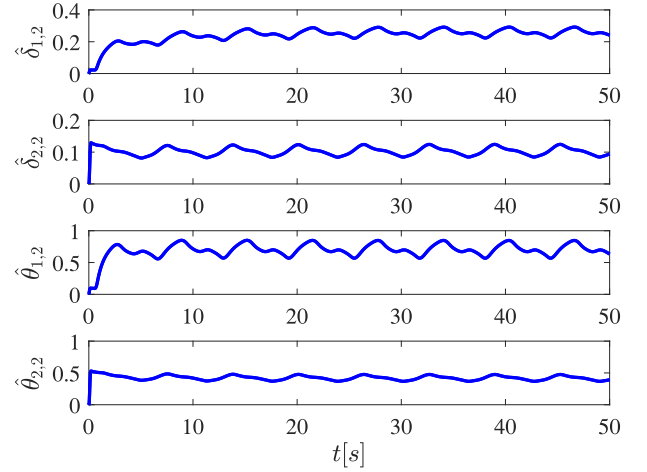
Fig. 8. Adaptation parameters \hat{\delta}_{1,2} , \hat{\delta}_{2,2} , \hat{\theta}_{1,2} , and \hat{\theta}_{2,2} .
