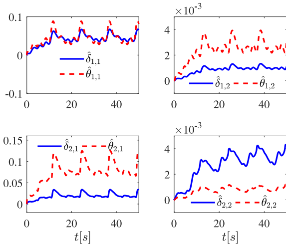
Fig. 3. Adaptation parameters \hat{\delta}_{1,1} , \hat{\delta}_{1,2} , \hat{\delta}_{2,1} , and \hat{\delta}_{2,2} .
