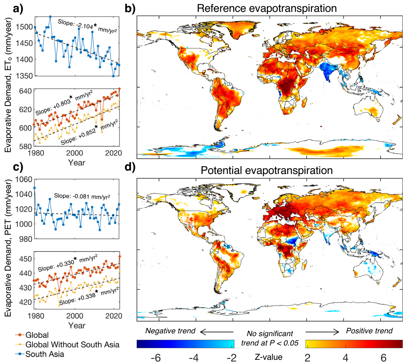
Fig. 2 | Trends in reference evapotranspiration (ET 0 ) and potential evapotranspiration (PET) show significant increases globally, except in South Asia. a, c Show time series of global, global excluding South Asia, and South Asia trends in annual ET 0 and PET (mm yr -1 ). b, d Spatial patterns of significant positive (red),
