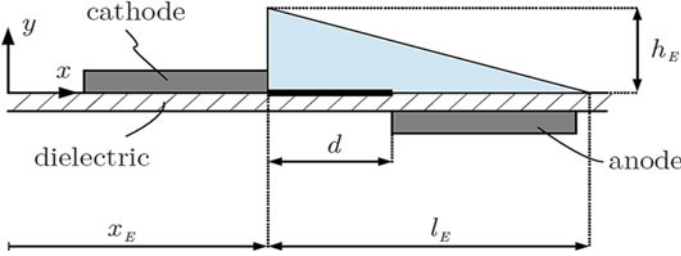
Fig. 19 Linearisation of the electric field
