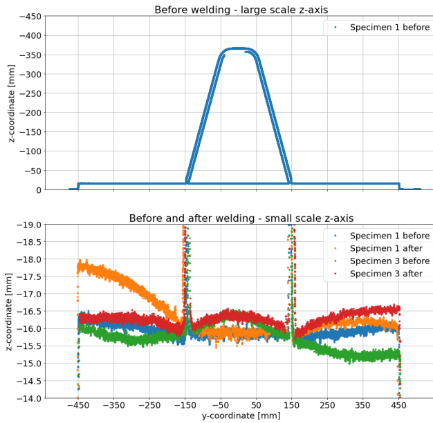
Figure 20. Raw data points along path 1
