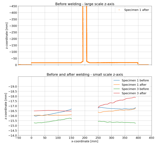
Figure 19. Z-coordinates of top of deck plate along path 3
