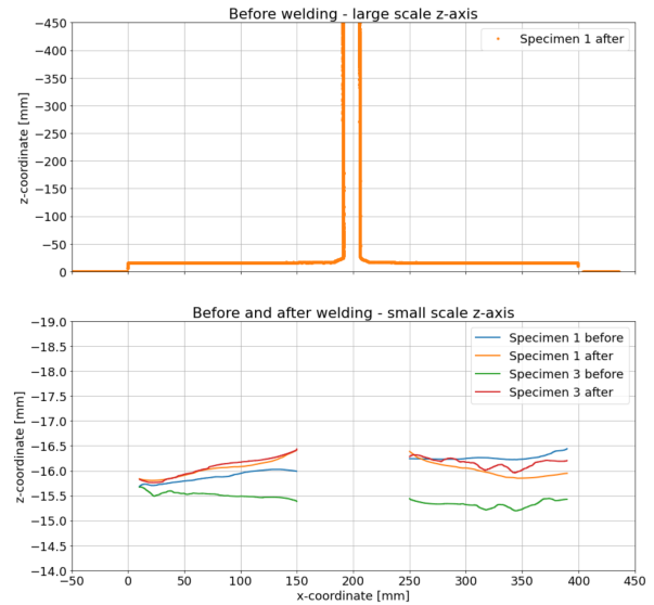
Figure 18. Z-coordinates of top of deck plate along path 2
