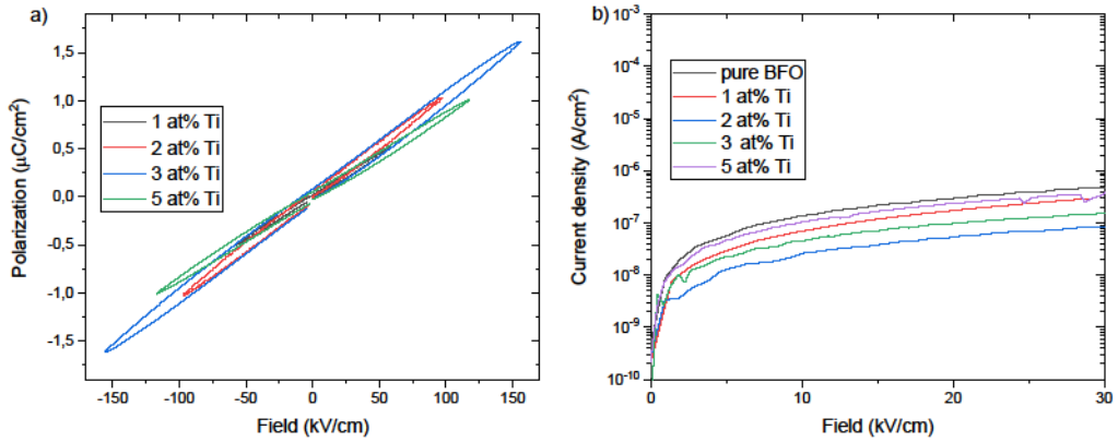
Figure 4.5 – a) Ferroelectric hysteresis loops and b) leakage current density of Ti-doped BFO ceramic samples
