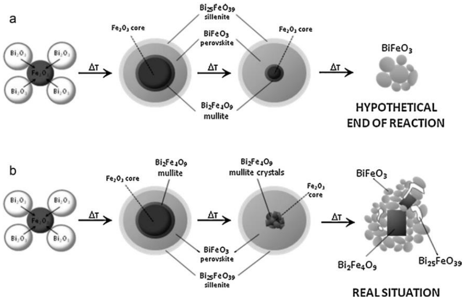
Figure 1.4 – Schematic diagram of the reaction paths in the solid-state synthesis of \text{BiFeO}_3 . (a) Hypothetical end of the reaction and (b) experimental situation for practical conditions. [31]
