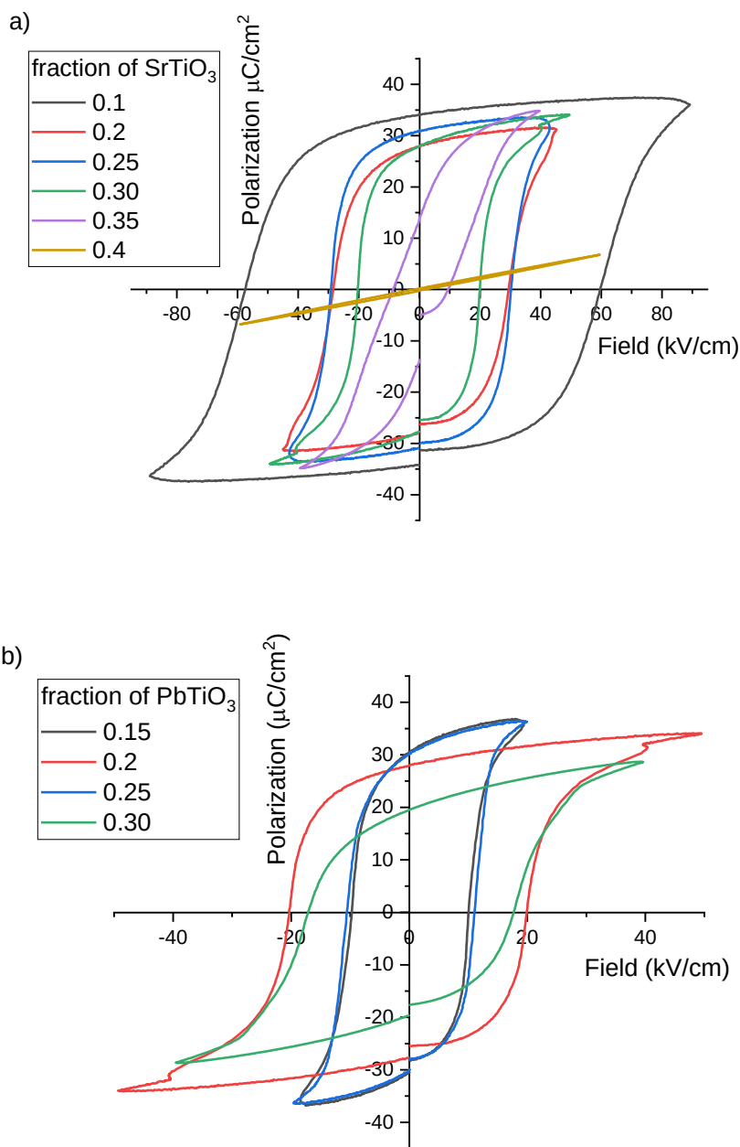
Figure 5.6 – Polarization-electric field (P-E) hysteresis loop of the BFO-PT-ST sintered ceramics with a) a fixed PT concentration (0.2PT) and b) a fixed ST concentration (0.3ST)
