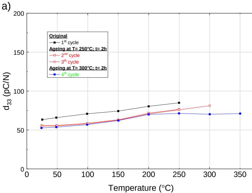
Figure 5.7 – Temperature dependence of the piezoelectric properties of the (0.8-x)\text{BFO-0.2PT-xST} ceramics for : a) x=0.1
