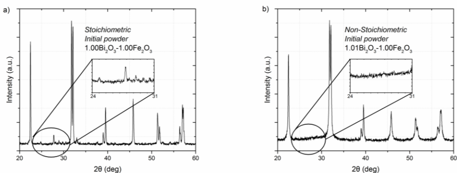
Figure 2.4 – X-ray diffraction analysis of samples prepared with and without the addition of extra bismuth. ( a - Equal amounts of iron and bismuth in the precursor; b - 1 mol% extra bismuth oxide added to precursor).
