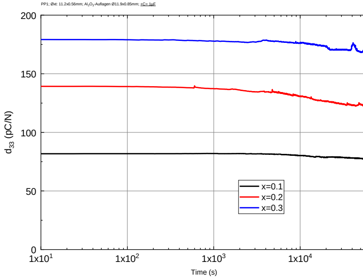
Figure 5.8 – Dependence of piezoelectric constant d_{33} on holding time at 300°C for (0.8-x)\text{BFO}-0.2\text{PT}-x\text{ST} ceramics
