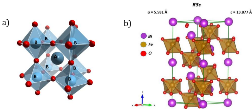
Figure 1.2 – a) perovskite type structures material is any material with a crystal structure having the formula ABO 3 (red spheres - oxygen), b) R\bar{3}c crystal structure of BiFeO 3
