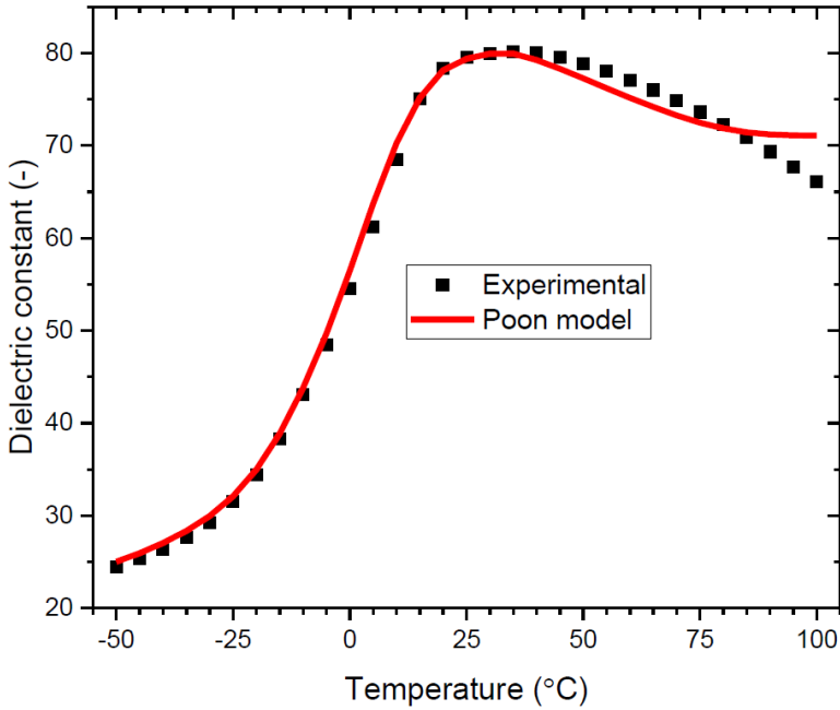
Figure 3.7 – Fitting of the temperature dependence of the dielectric constant at 1 kHz for the 50 vol% \text{BiFeO}_3 -PVDF composite to the Poon model using the data from Figure 3.3
