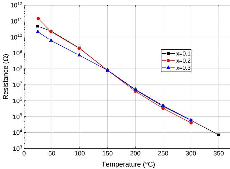
Figure 5.9 – Temperature dependence of electrical resistance for (0.8-x)\text{BFO}-0.2\text{PT}-x\text{ST} ceramics
