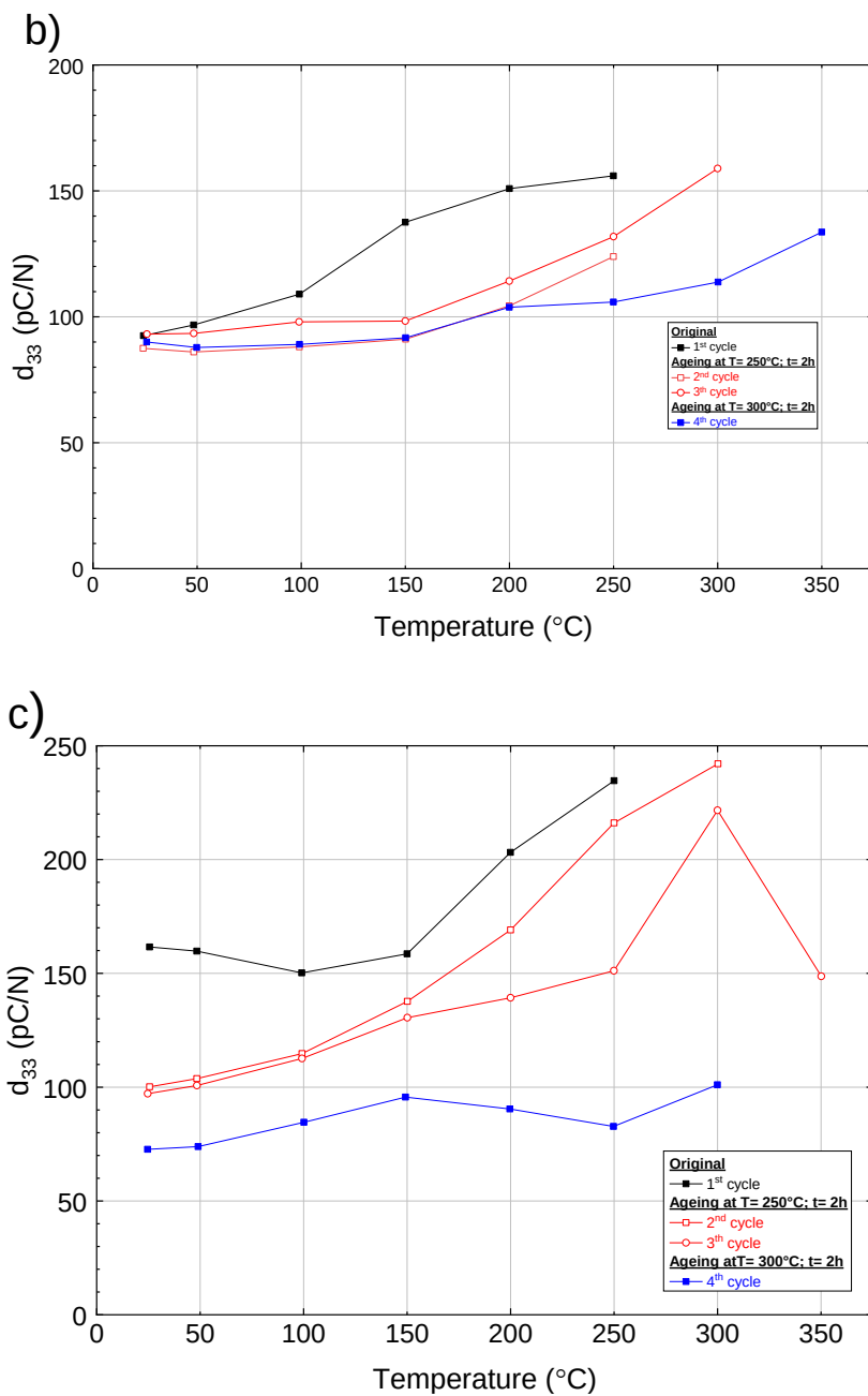
Figure 5.7 (continued) – Temperature dependence of the piezoelectric properties of the (0.8-x)BFO-0.2PT-xST ceramics for : b) x=0.2 ; c) x=0.3
