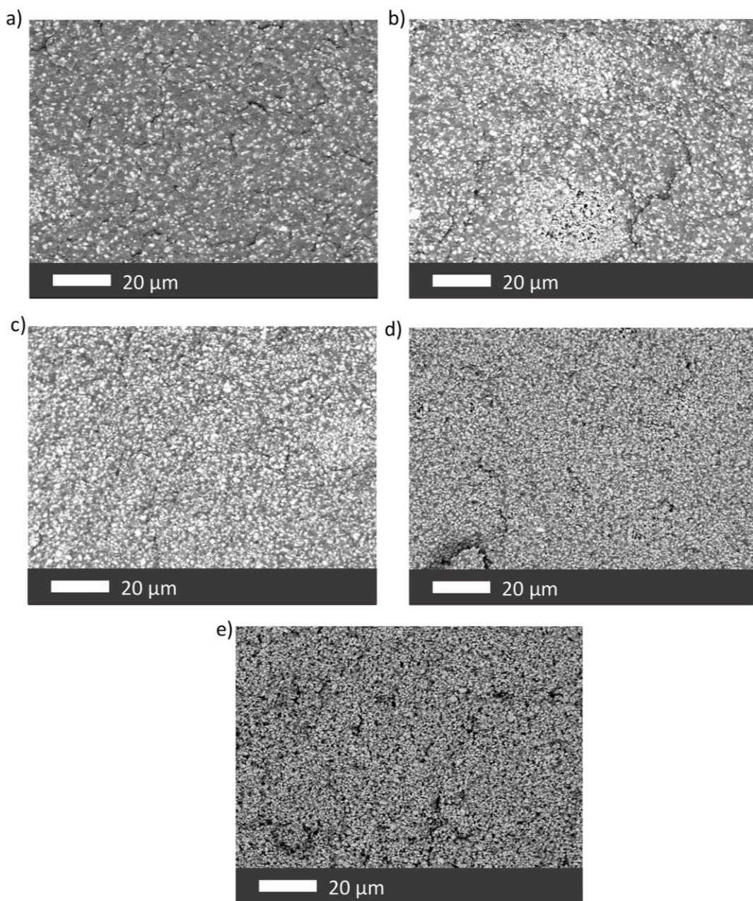
Figure 3.2 – SEM picture cross-section of \text{BiFeO}_3 -PVDF composites: a) 20 vol%; b) 30 vol%; c) 40 vol%; d) 50 vol%; e) 60 vol%
