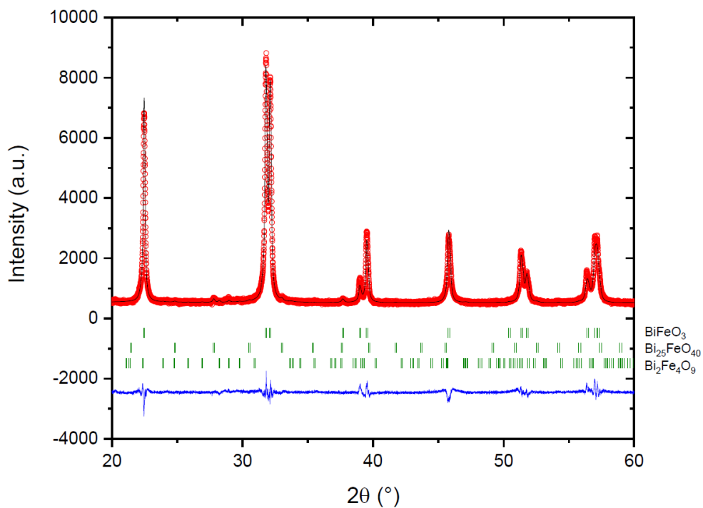
Figure 4.1S – Rietveld refinement of the XRD pattern of undoped BFO.
