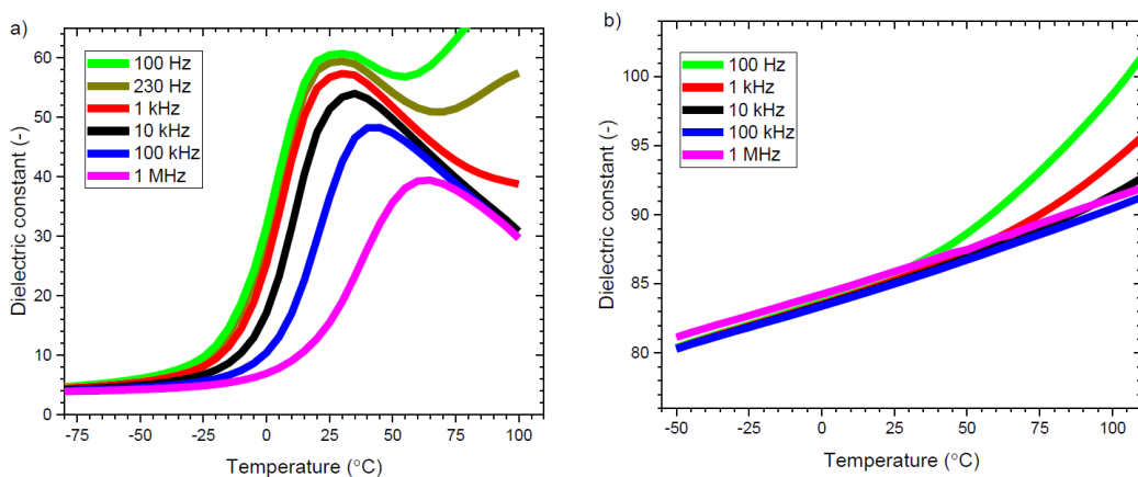
Figure 3.3 – Dielectric constant as a function of the temperature: a) PVDF terpolymer film and b) sintered BiFeO 3 bulk ceramic
