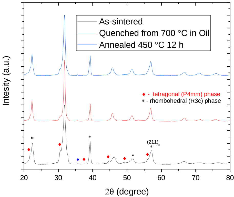
Figure 6.2 – X-ray diffraction patterns of the as-sintered, oil quenched from 700 °C and 12 h, 450 °C annealed after oil quenching samples
