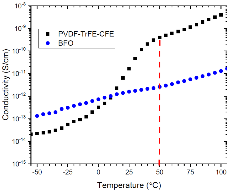
Figure 3.4 – DC conductivity PVDF-terpolymer film and bulk \text{BiFeO}_3 ceramic as a function of the temperature
