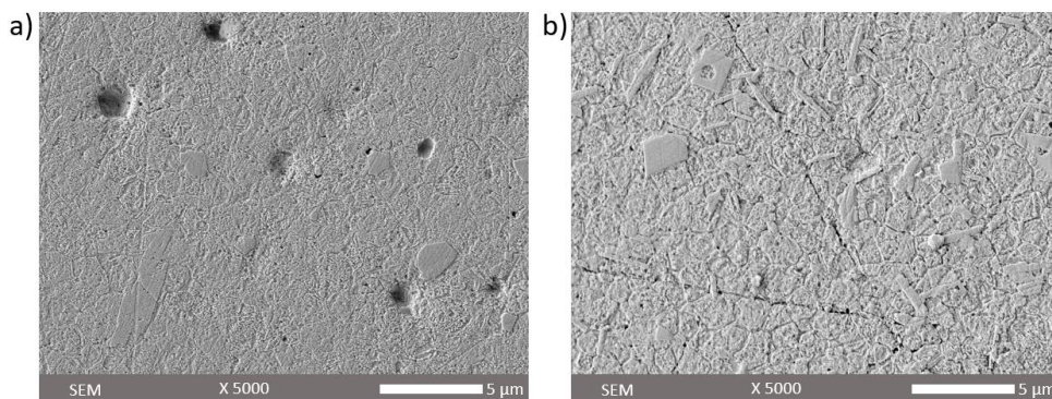
Figure 6.3S – SEM picture of a polished a) quenched and b) annealed sample after chemical etching (both samples over etched)
