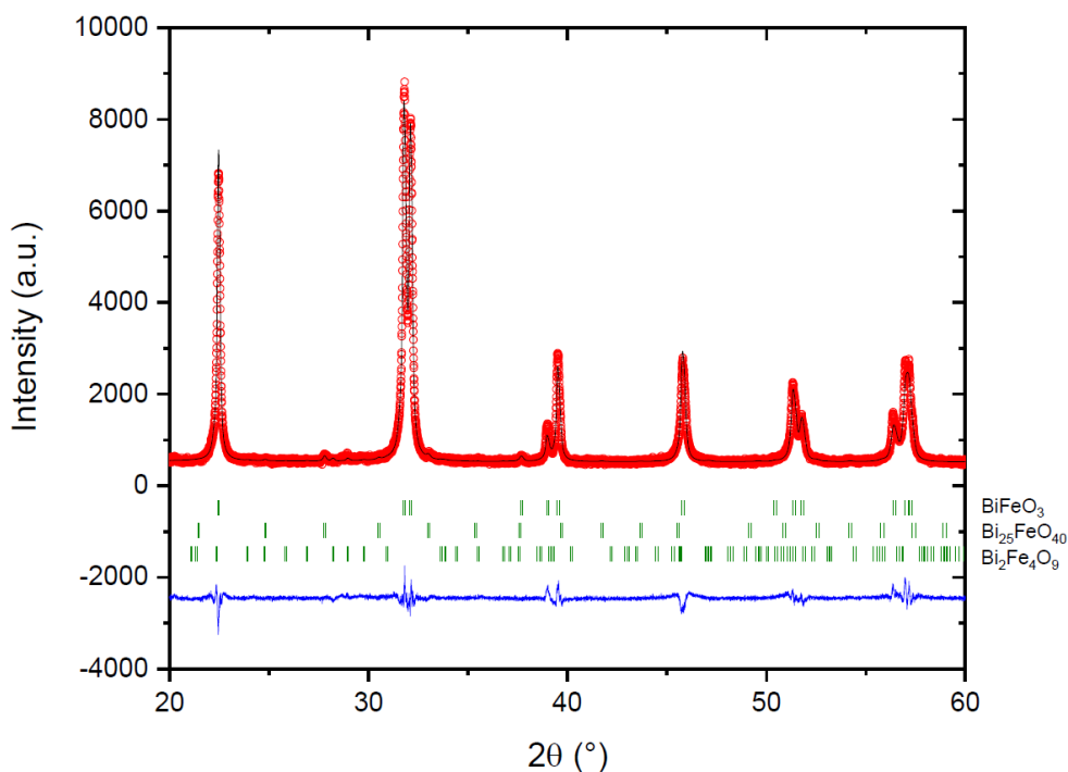
Figure 3.1 – Rietveld refined XRD patterns of the calcined \text{BiFeO}_3 ceramic powder. R-Bragg for the main phase is 3.21 %.
