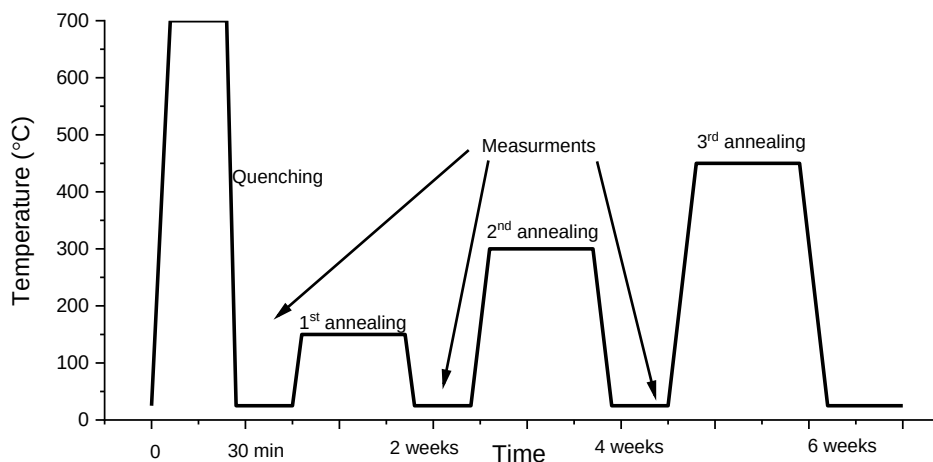
Figure 6.4S – Thermal history of annealing procedure.
