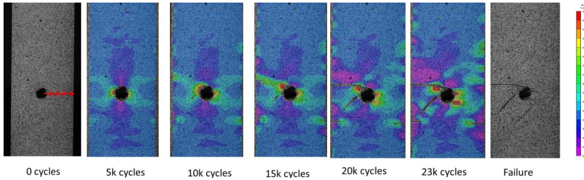
Figure 2. The \varepsilon_{yy} strain distribution (load direction).
