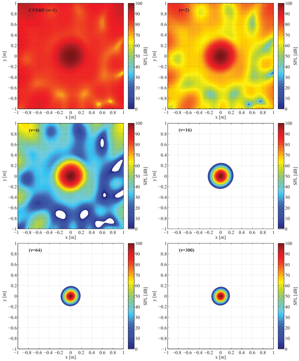
Fig. 2: Comparison between the obtained source plots for a single 100 dB source situated at (0, 0) m emitting at 1000 Hz and 1 m from the array, using from left to right and from top to bottom: CFDBF algorithm ( \nu = 1 ) and functional beamforming algorithm for different exponent values:
