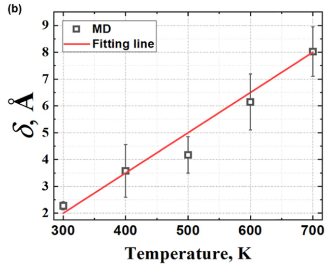
Figure 15. (a) Trajectory lines of atom movements at different temperatures for the polycrystals with \sim 14 nm grains. (b) GBs thickness at various temperatures for different grain sizes.
