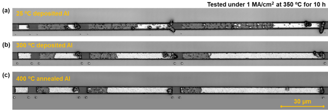
Figure 8. Electromigration results for Al stripes with different deposition temperatures tested under 1 MA cm -2 at 350 °C for 10 h.
