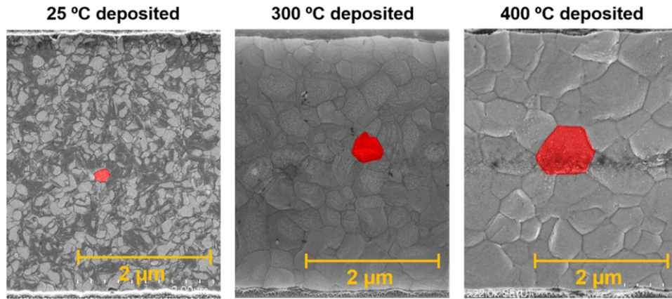
Figure 9. SEM images for Al stripes deposited at 25 °C, 300 °C, 400 °C, respectively.
