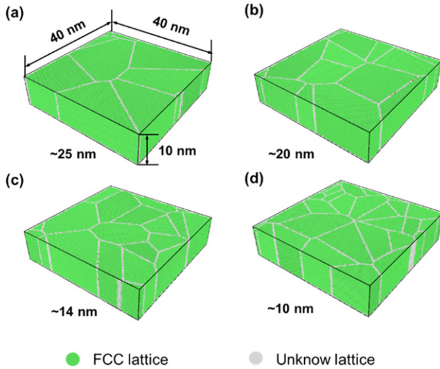
Figure 2. Polycrystalline models with grain sizes of (a) 25 nm, (b) 20 nm, (c) 14 nm, and (d) 10 nm. The green region represents the atoms in grains with fcc lattice structure and the grey region represents the atoms in GBs with the irregular lattice structure.
