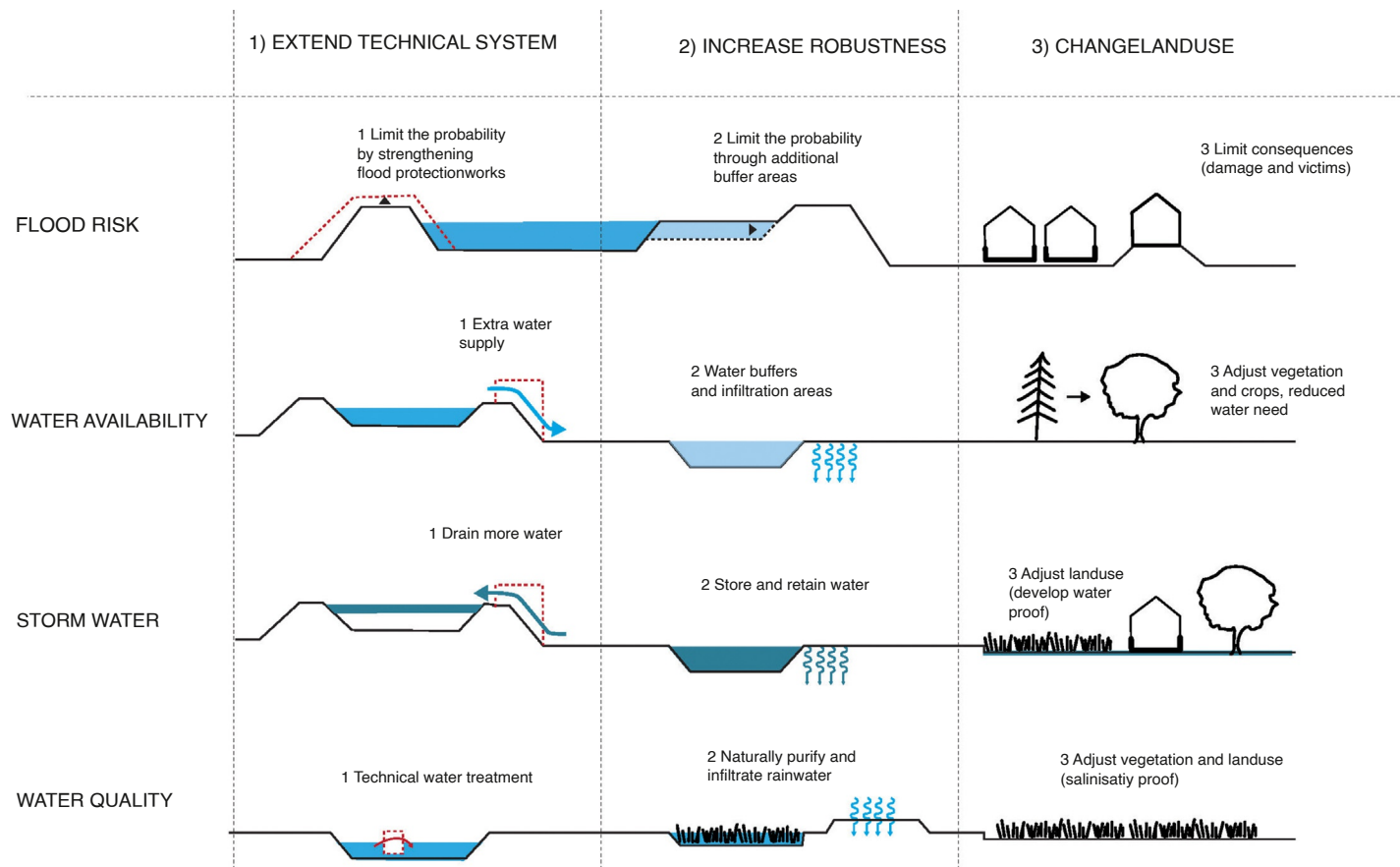
Fig. 3 Scheme showing different options for extending the water system: Expanding the technical system (Column 1), improving the robustness of the system (Column 2), or changing the land use (Column 3). (Image by Defacto Urbanism.)
