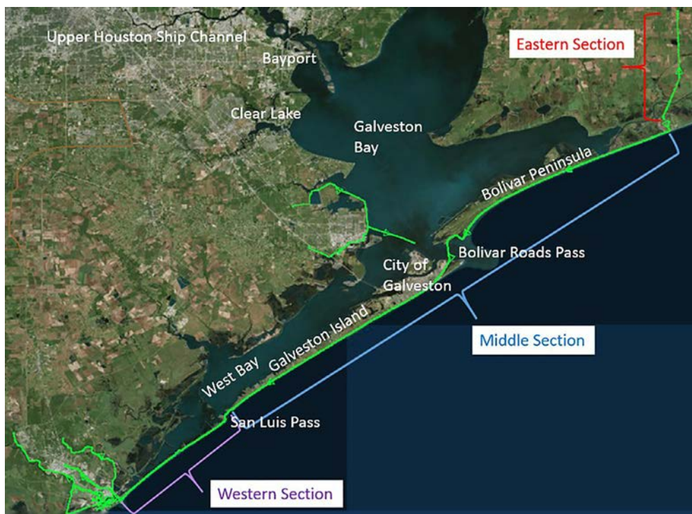
Fig. 1 Location map for the Houston-Galveston region, and footprint of the Ike Dike coastal spine concept.
