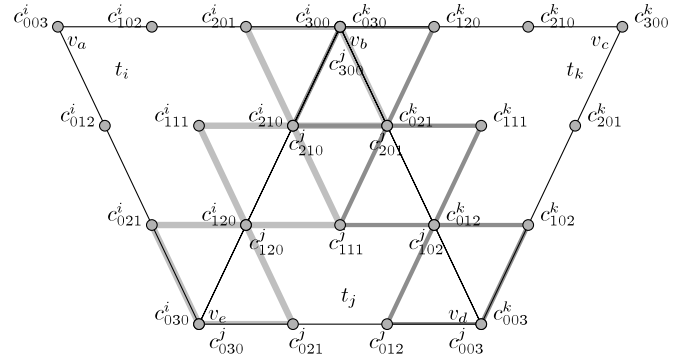
Fig. 1. B-net for third degree basis function on 3 simplices together with C^1 continuity structure (bold lines).
