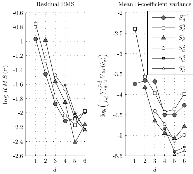
Fig. 3. RMS of the residual r(x_1, x_2) (left) and mean B-coefficient variances (right) for the different spline spaces.
