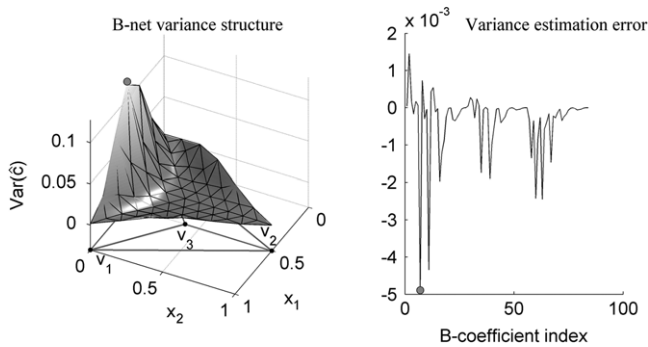
Fig. 5. Estimated (= solid) and simulated (= wireframe) B-coefficient variance structure (left) and the error in the variance estimation (right). The dot corresponds to the B-coefficient at which the largest error between estimated and simulated variance occurs.
