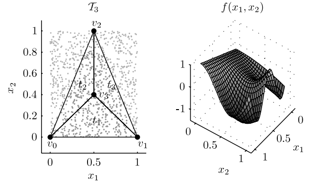
Fig. 2. Triangulation \mathcal{T}_3 and identification dataset (left) and data generating function f(x_1, x_2) (right).
