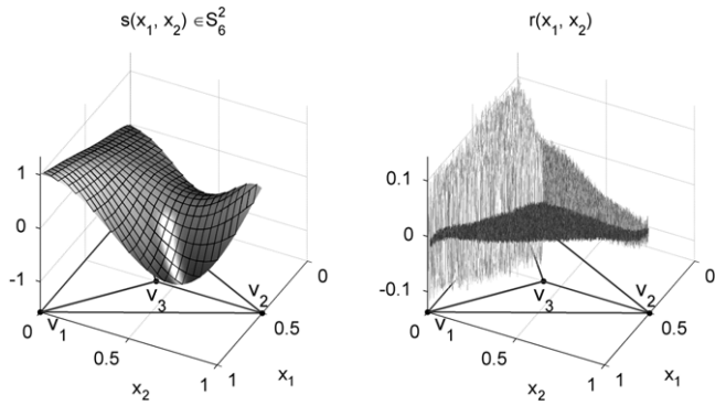
Fig. 4. Sixth degree spline function with C^2 continuity (left) and model error (right).
