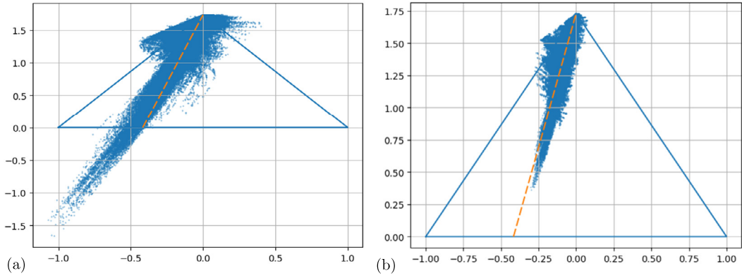
Fig. 3. Modeled anisotropy tensor at each mesh cell placed in the barycentric map for 100 random vectors \Theta_{ij}^{b\Delta} sampled using uniform Latin Hypercube sampling. (a) sampling in range [-7, 7]^{18} . (b) Sampling in range [-2, 2]^{18} .
