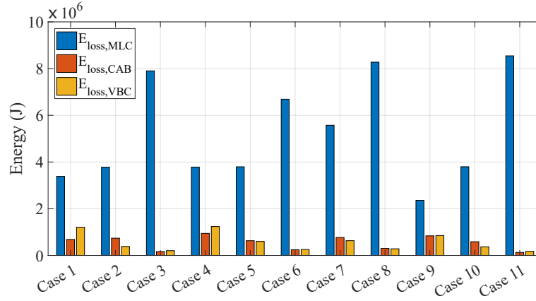
Figure 14: Loss distribution for different cases of the Aramis building, evaluated on August 30, 2019.
