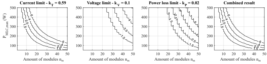
Figure 9: Separate and combined results for cable selection in a +100 V/0/-100 V system as a function of the total amount of modules in the system ( n_m ) and the maximum MLC output power ( P_{MLC,max} ). The lines indicate the transition from one cable cross section to another.
