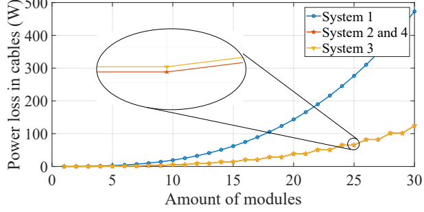
Figure 4: Cable losses as a function of the amount of modules for different network configurations ( R = 0.1 \, \Omega and I_{MLC} = 0.5 \, A ). A magnification has been included to highlight the minor difference between system 3 and systems 2/4.
