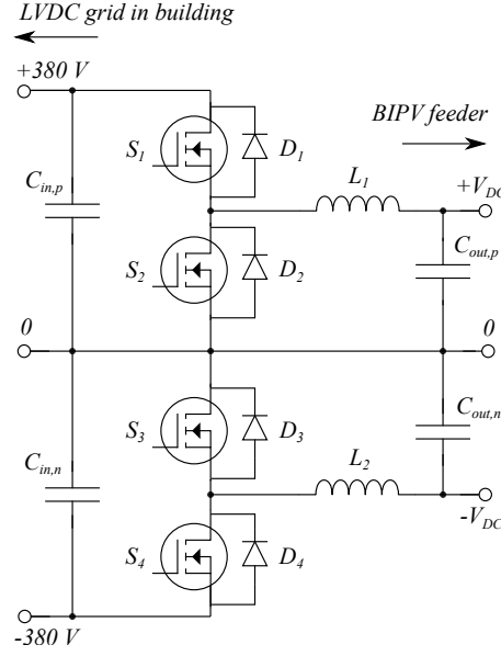
Figure 10: Three-level boost converter topology, used as a VBC to couple the BIPV feeder with the LVC grid inside the building.
