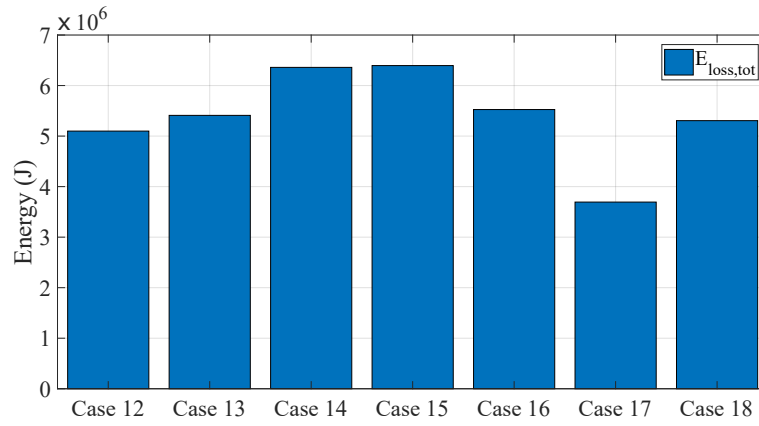
Figure 16: Total energy loss for different cases of the South Tower building, evaluated on August 30, 2019.
