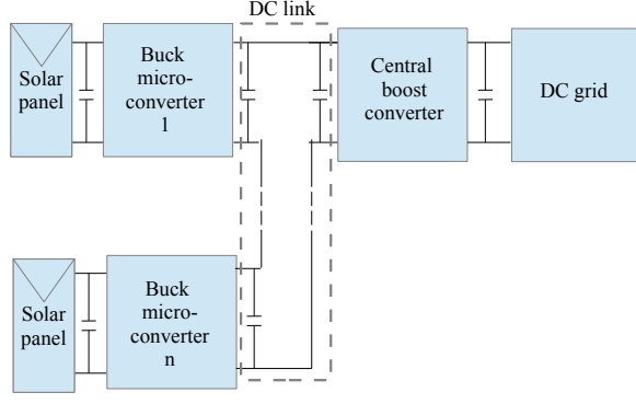
Fig. 10. Buck microconverters and boost central converter topology
