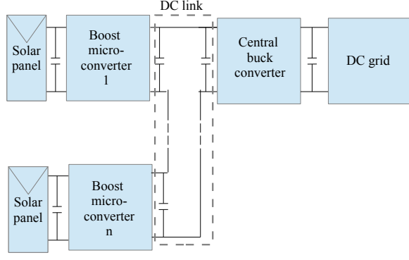
Fig. 6. Boost microconverters and buck central converter topology
