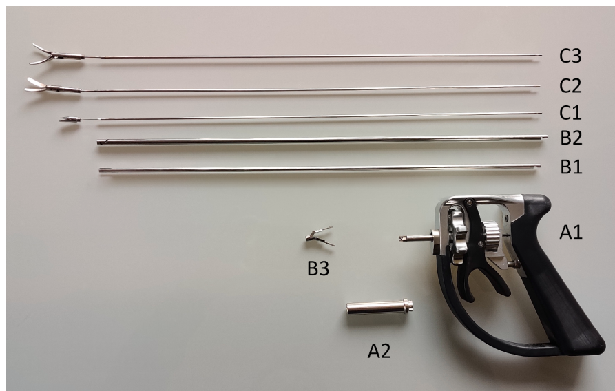
Fig. 5. The device completely disassembled. A1: Handle, A2: Shaft Busing, B1: Middle Shaft, B2: Outer Shaft, B3: SATA-joint, C1/C3: Push-pull rod with a clip applicator, cutter and grasper tip respectively.
