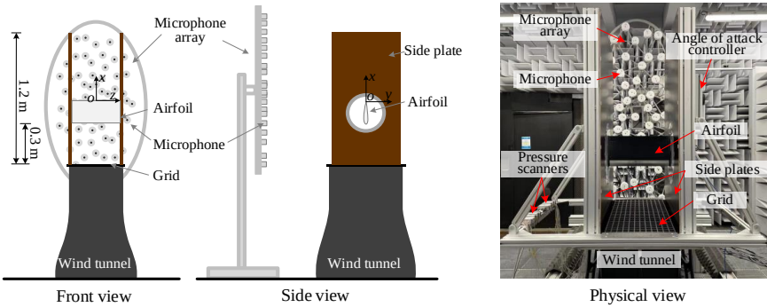
Figure 5.1: Experimental setup.
