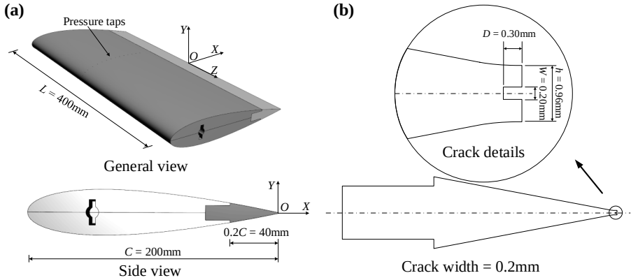
Figure 3.1: Experimental setup.
