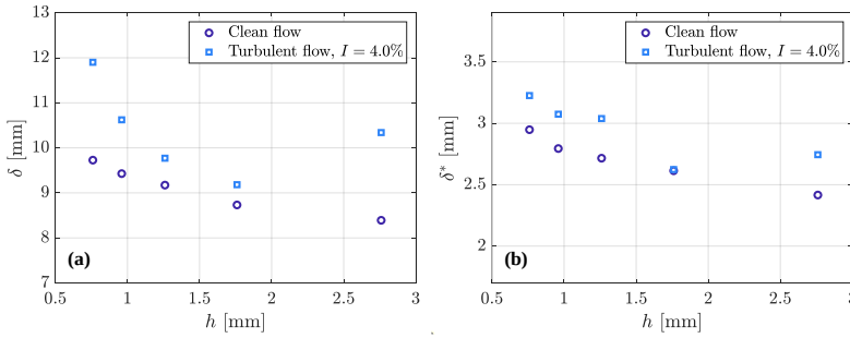
Figure 4.11: Boundary layer thickness and displacement thickness at the trailing edge for different crack sizes for 35 m/s inflow and zero angle of attack condition: (a) boundary layer thickness and (b) displacement thickness.
