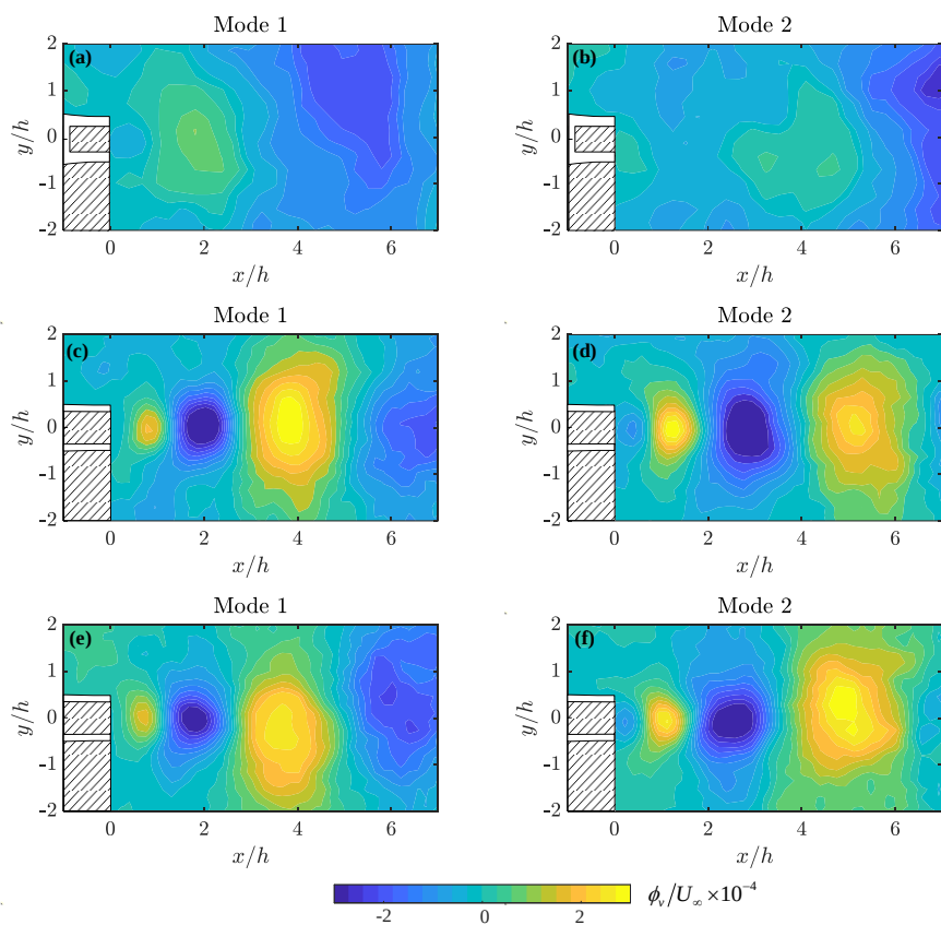
Figure 4.14: First two POD models of the \nu component for the cases: (a) and (b) 1.0 mm crack case for clean inflow condition; (c) and (d) 2.0 mm crack for clean inflow condition; (e) and (f) 2.0 mm crack for turbulent inflow condition. The white blocks are the trailing edges and the shaded sections are the shadow areas of the laser.
