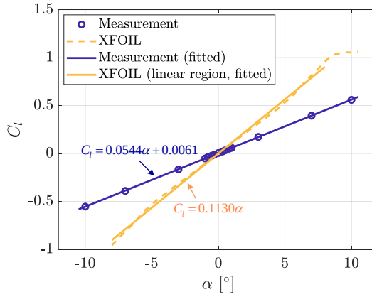
Figure 3.3: The relationships between C_l , \alpha and \alpha^* from the measured data and XFOIL.
