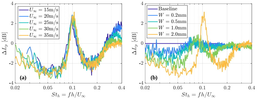
Figure 3.8: The relationships between \Delta L_p and St_h with AoA of 0^\circ : (a) under different mean flow velocities when crack width is 2.0 mm; and (b) under different crack sizes when mean flow velocity is 35 m/s.
