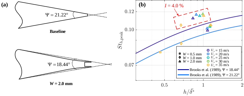
Figure 4.19: Comparison with the model developed by Brooks et al.: (a) definition of solid angle for baseline and cracked cases; (b) dependence of the peak Strouhal number versus the ratio of trailing edge thickness to boundary layer displacement thickness. The points outside the dashed box are for clean inflow cases. Solid lines are obtained using the semi-empirical law reported by Brooks et al. for the two different values of the solid angle shown in (a).
