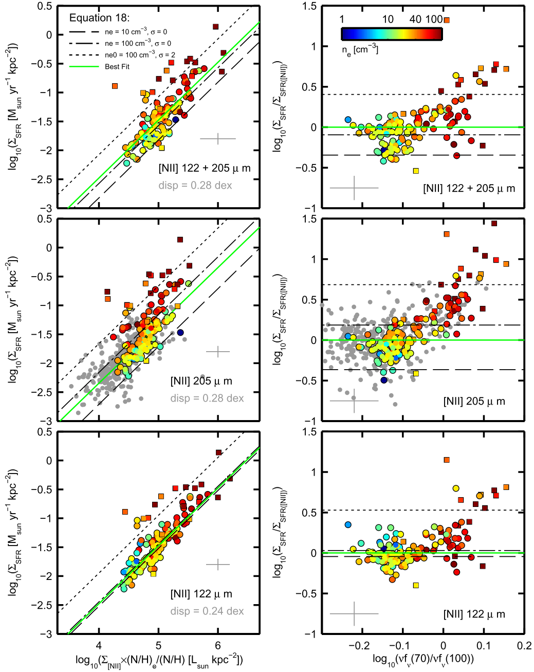
Figure 8. Left panels: star-formation rate surface density ( \Sigma_{\text{SFR}}(\text{H}\alpha + 24 \mu\text{m}) ) versus the combined ( \Sigma_{122+205} ) and individual ( \Sigma_{122} and \Sigma_{205} ) [N II] line surface brightness scaled by the nitrogen abundance factor (\text{N}/\text{H})_o/(\text{N}/\text{H}) . Each point represents a 17'' region selected from the 21 BTP galaxies. The error bars in the bottom corner show the typical uncertainty on the measurements. For regions with [N II] 122/205 line ratios available, the color represents the electron density. In the case of the [N II] 205 \mu\text{m} line, the gray points correspond to 366 additional regions that lie outside the KINGFISH/PACS coverage and therefore lack [N II] 122 \mu\text{m} observations. We also show regions with deprojected distances to the center smaller than 400 pc as squares. The green solid line corresponds to the best fit through the data for a fixed slope of one. The rest of the lines correspond to the results from Equation (18) for different assumptions on the electron density distribution parameters n_e and \sigma . Right panels: ratio between \Sigma_{\text{SFR}} measured using \text{H}\alpha + 24 \mu\text{m} and the [N II] lines (based on the best linear fit) as a function of infrared color and electron density. We also include the predictions from Equation (18) shown in the left panels. We observe a systematic increase of the \Sigma_{\text{SFR}}/\Sigma_{\text{SFR}}(\text{N II}) ratio as a function of infrared color and electron density. As predicted by Equation (18), these deviations could be associated with a higher density distribution parameter \sigma or to electron densities higher than the critical density of the [N II] lines. We observe the largest deviations from the linear fit for the [N II] 205 \mu\text{m} line, which is expected given that the critical density of this line is about six times lower than the critical density of the [N II] 122 \mu\text{m} transition.
