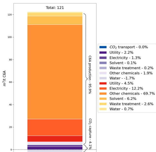
Fig. 6. Breakdown of water consumption of the MES route with economic allocation.
