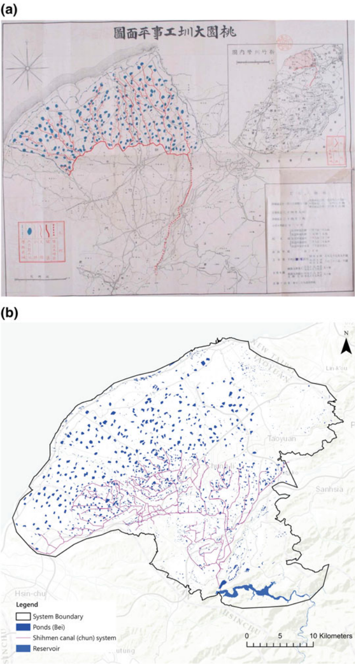
Fig. 3 Canal systems and Reservoir on Taoyuan tableland: a Taoyuan Main Canal fortification plan in the 1920's (above), b Shihmen Reservoir and Shihmen Main Canal system in 2016; released under a Creative Commons Attribution-NonCommercial-NoDerivatives 4.0 International License
