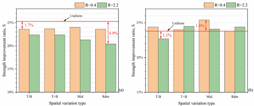
Fig. 4. Strength improvement ratio in extension of (a) bridging and (b) contact cementing samples with different inhomogeneity characteristics.
