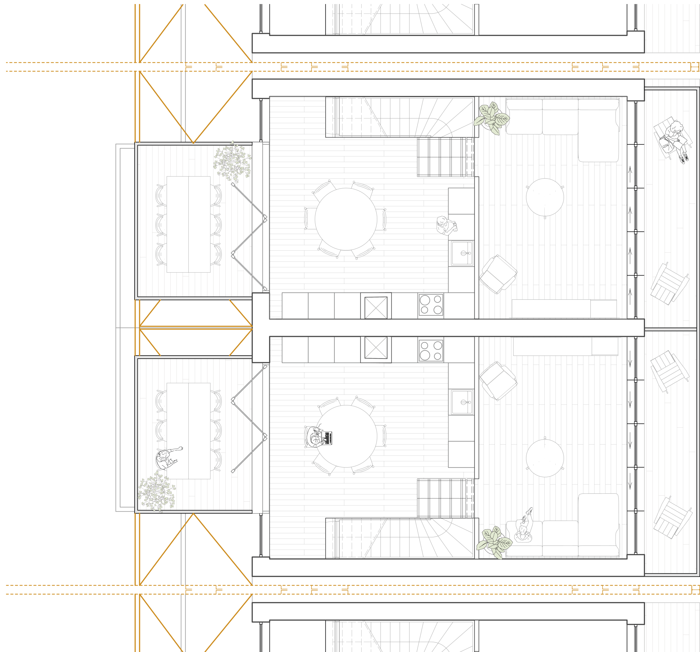
Floorplan - First floor
