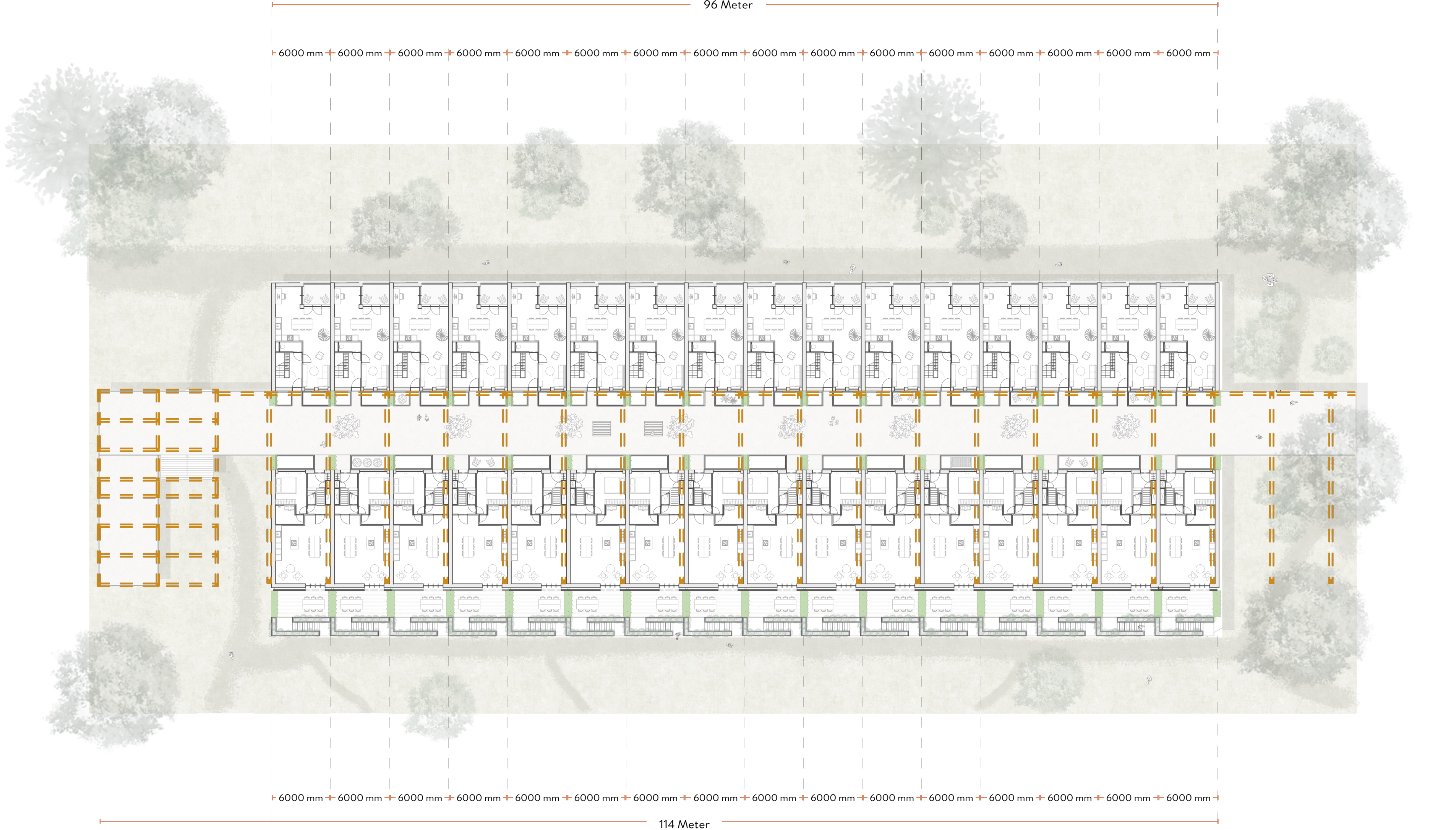
Floorplan - Kloos level
