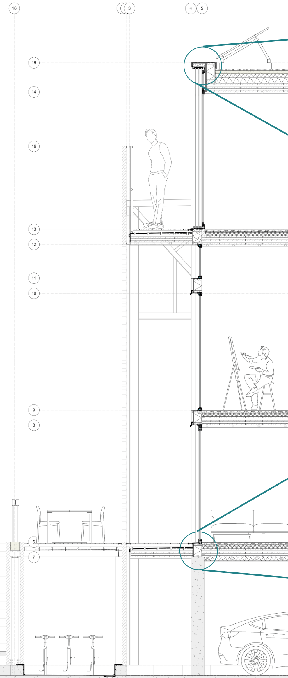
Facade fragment
