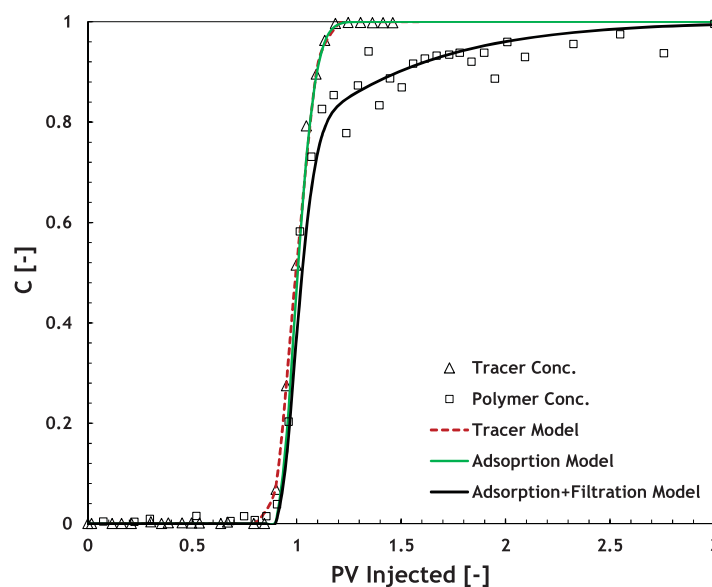
Figure 13. Comparison of the model with the experimental data (hydrolyzed polyacrylamide, HPAM, flow through a core with length of 30.5 cm, diameter of 3.81cm, k = 2500 mD, and \phi = 0.23 ). The polymer was injected with velocity of 2 ft/d. The fit to the tracer data was obtained with a dispersivity length of 0.1 mm. The fit to the polymer data is obtained by setting \lambda_0 = 0.55 \text{ ft}^{-1} and \sigma_{\text{max}} = 0.016 \text{ m}^3/(\text{m}^3 \text{ PV}) . Data from Lee [2015].
