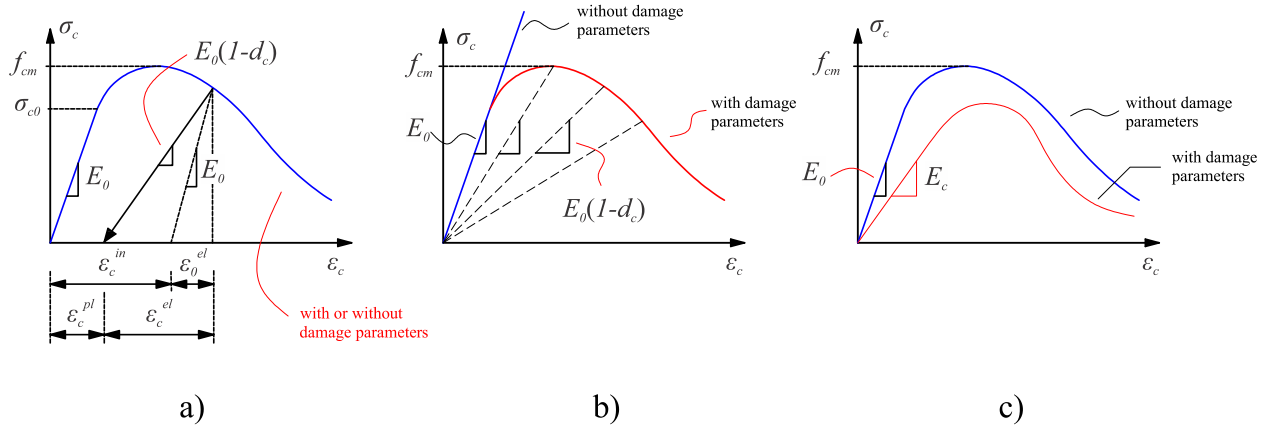
Fig. 3. A) stress-strain behavior in compression considered in the Concrete Damaged Plasticity (CDP); b) stress-strain behavior model with and without damage parameters considered by pure damage models; c) erroneous assumption of stress-strain behavior when considering damage parameters.
