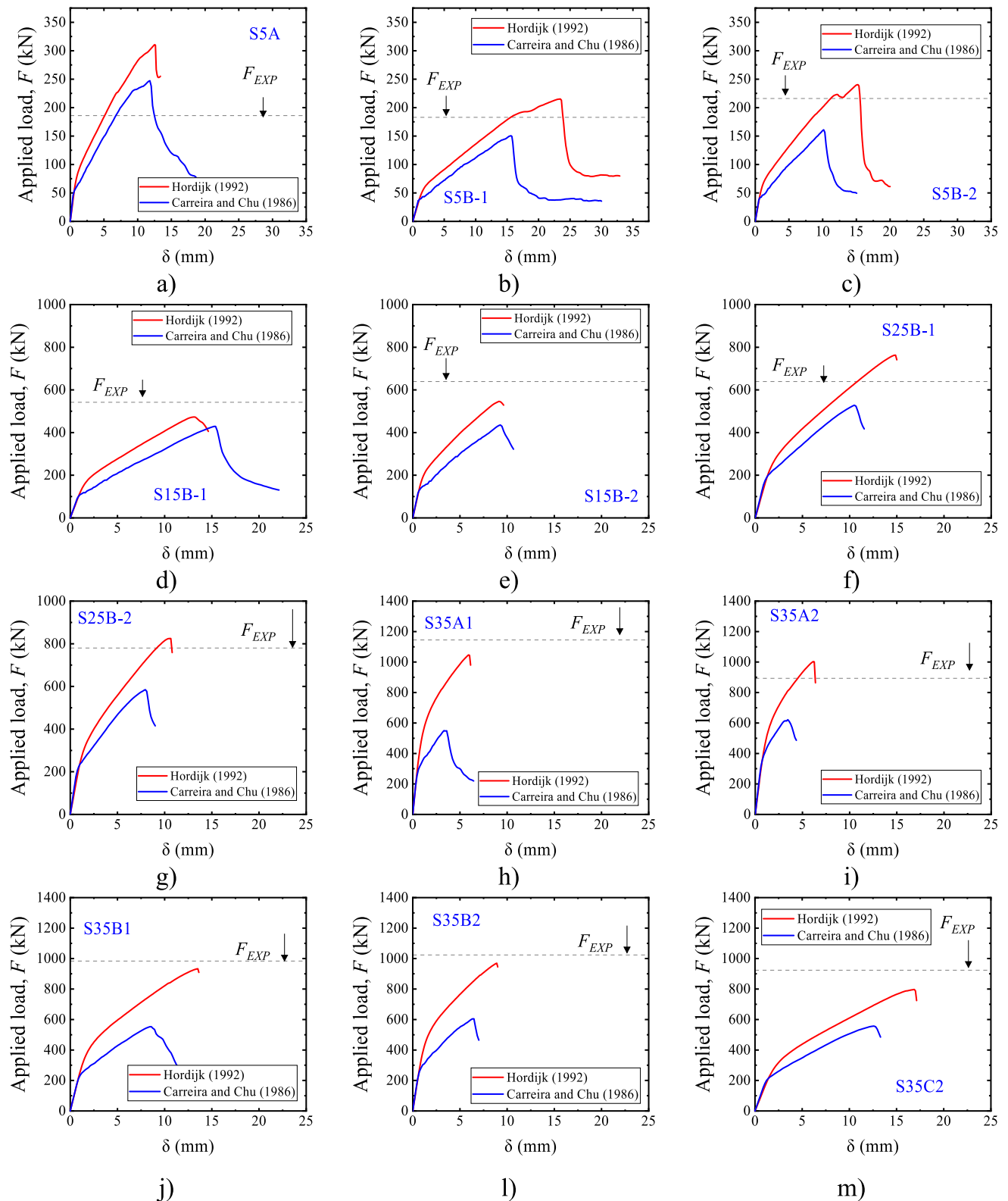
Fig. A3. Influence of the tensile stress-strain behavior.
