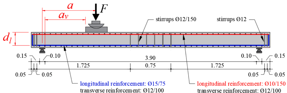
Fig. 6. Reinforcement layout of simply supported slabs with l_{total} = 4.4 m tested by Reißen, Classen and Hegger [8]. Dimensions in m.
