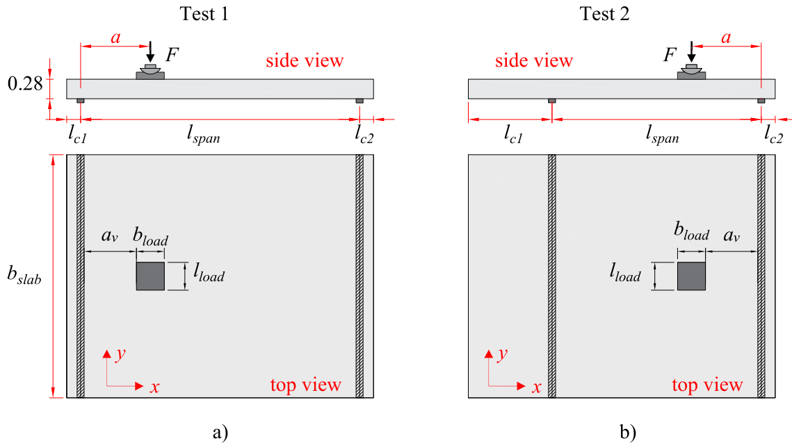
Fig. 4. Schematic view of the geometry of the one-way slabs tested by Reiß, Classen and Hegger (2018) evaluated in this study: a) layout of the first test on the specimens and; b) layout of the second test on the specimens. Source: Adapted from Reiß, Classen and Hegger [8].
