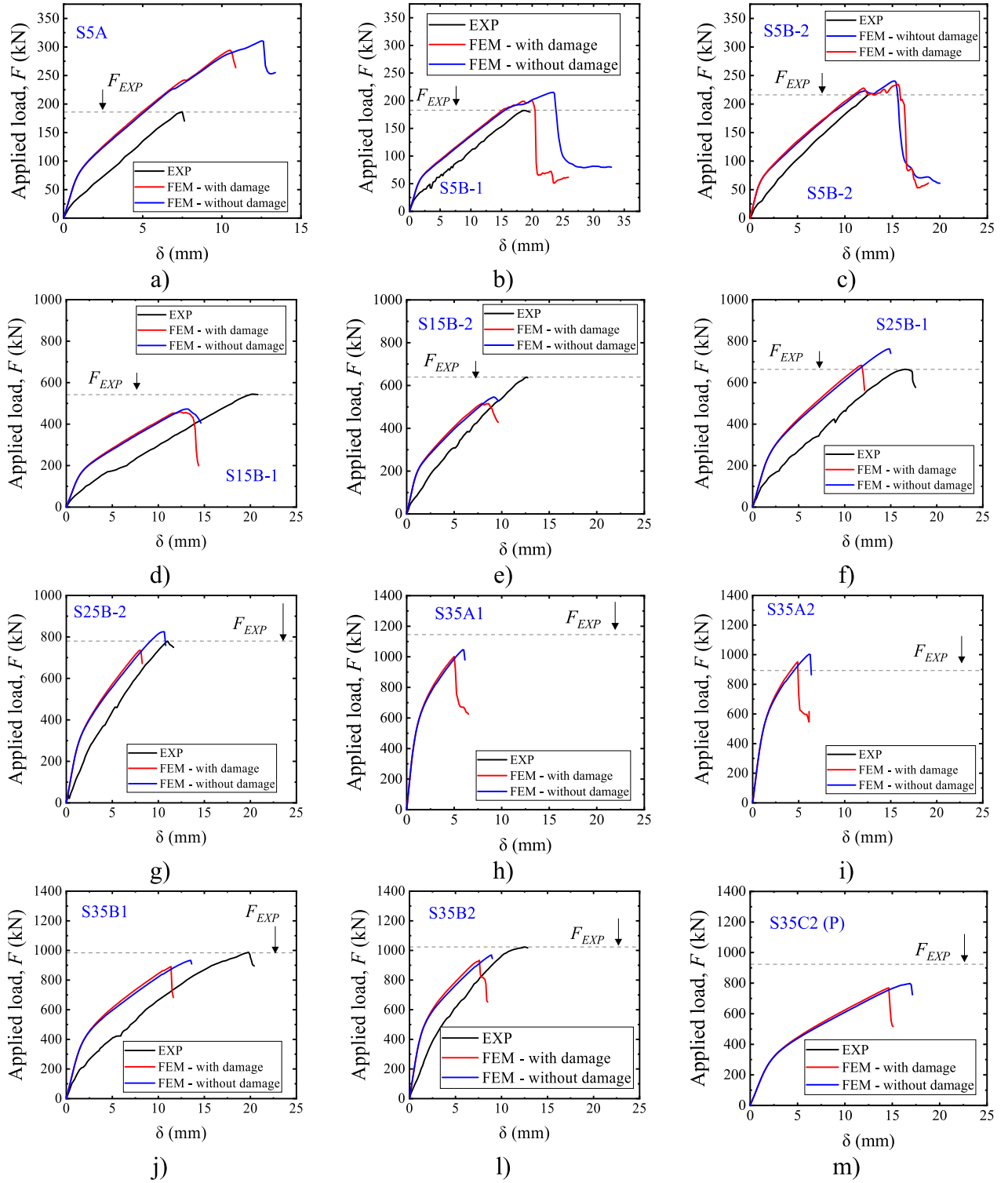
Fig. A1. Influence of including or not the damage parameters in the load \times displacement curves of the numerical simulations.
