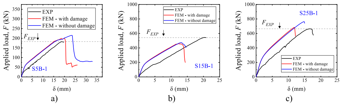
Fig. 14. Influence of including or not the damage parameters in the load \times displacement curves of the numerical simulations. Note: graphs from other tests can be consulted in the Appendix.
