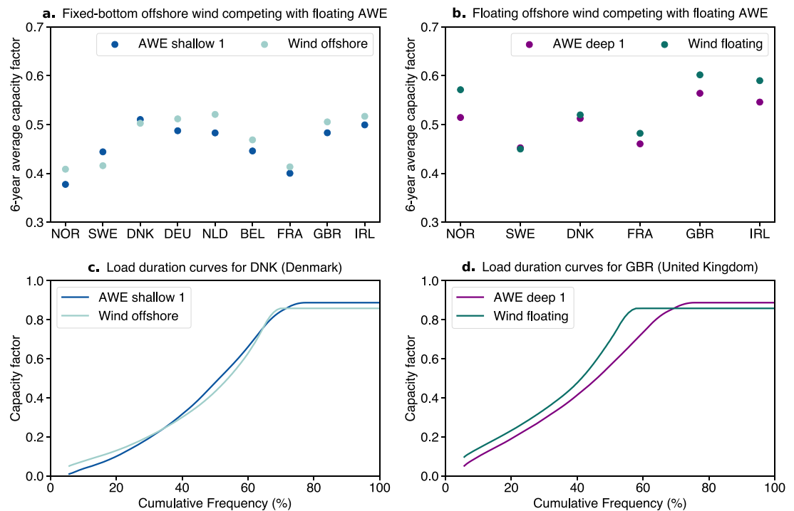
Figure 7. Six-year average nationwide capacity factors for shallow water AWE vs. fixed-bottom offshore wind (a), and deep water AWE vs. floating offshore wind turbines (b), as well as the corresponding load duration curves for Denmark (c) and the United Kingdom (d).
