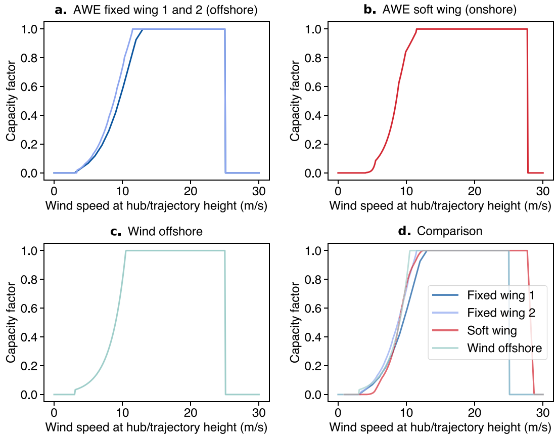
Figure 3. Power curves of considered AWE systems compare with the conventional offshore wind power curve used: Fixed-wing 1 and 2 (used offshore) (a), Soft wing (used onshore) (b), and conventional offshore wind (c). A comparison is also depicted (d), outlining the differences between the different curves.
