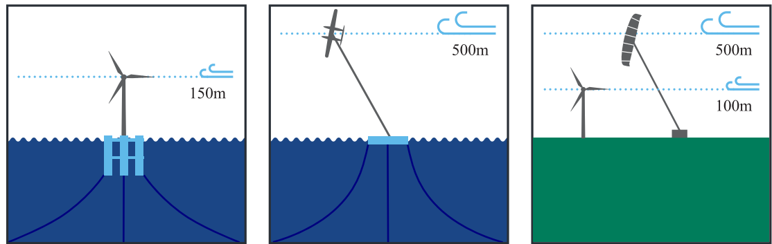
Figure 1. Floating offshore horizontal-axis wind turbine (left), floating offshore fixed-wing AWE energy system (centre), and onshore soft-wing AWE system with a wind turbine for reference (right).
