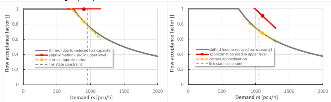
Fig. 12. \alpha_{23}(D_{rs}) , sensitivity approximations and link state constraints for not constraining (left) and constraining (right) cases when effective turn capacity is reduced to 750 pcu/h.
