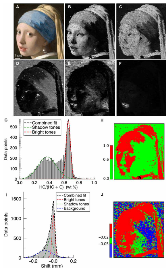
Fig. 3. Results obtained with MA-XRPD reflection mode. (A) Optical photograph of the analyzed area. (B to F) Distribution images obtained with reflection MA-XRPD showing the scaling parameter for every pixel. Higher scaling parameter values are represented by a brighter color. (B) Hydrocerussite, (C) cerussite, (D) calcite, (E) palmierite, and (F) cinnabar. (G) Histogram for the w_{HC}/(w_{HC} + w_C) ratios. The black dashed line represents the combined contribution of both Gaussian curves. (H) Corresponding RGB image for (G). (I) Histogram for the average depth of hydrocerussite relative to the average depth of cerussite. (J) Corresponding RGB image for (I). Images were scaled independently of each other: Intensities should not be directly compared. Photo credit: René Gerritsen, Art & Research Photography and Mauritshuis.
