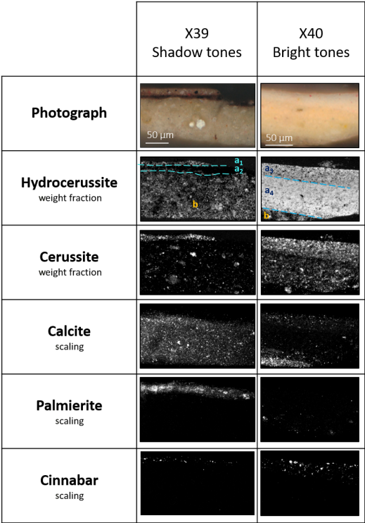
Fig. 2. Crystalline phase distributions obtained by \mu -XRPD for two paint cross sections collected from the Girl 's face. For hydrocerussite and cerussite, the weight fractions were calculated in every pixel of the image. For calcite, palmierite, and cinnabar, a scaling parameter is displayed instead to improve the qualitative readability of the maps. Brighter areas indicate a higher weight fraction or scaling parameter value. The intensity was scaled independently for each image to improve readability: Intensities should not be directly compared. The scan parameters and size of the scanned areas are shown in table S1.
