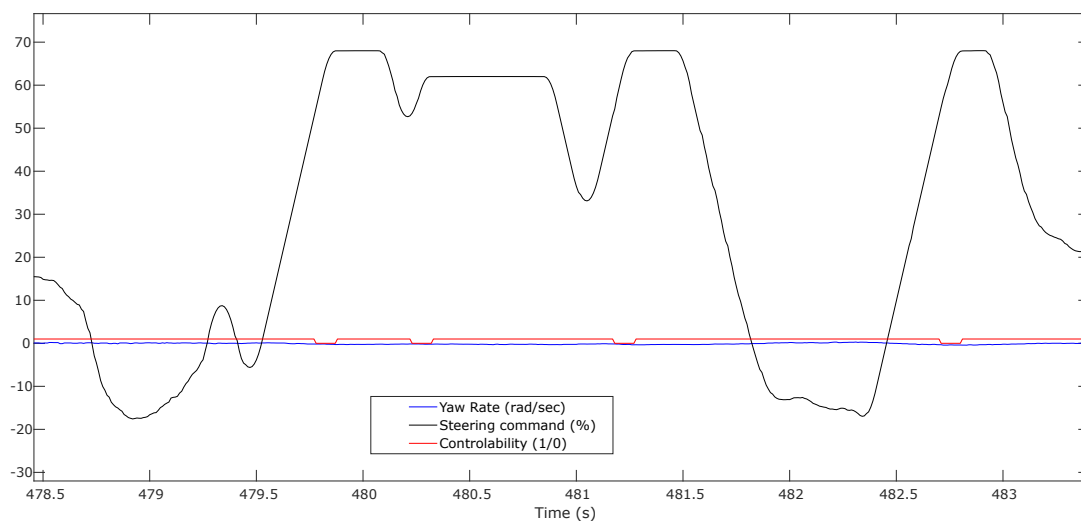
Figure 9. Steering input command (%), yaw-rate response (rad/sec) and simulated controllability anomaly result (1/0) during the second stall case
