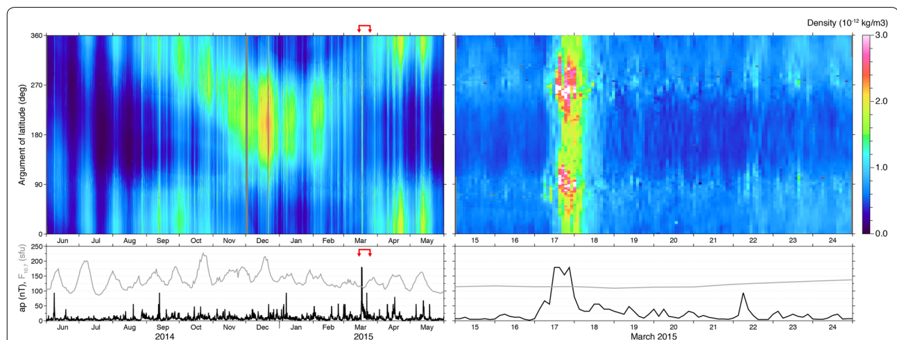
Fig. 12 Swarm C densities as a function of time and argument of latitude ( upper panels ) and solar and geomagnetic activity indices F_{10.7} and a_p ( bottom panels ). The left panels show the entire year of data that has currently been processed. The right panels zoom in on the 10 days surrounding the March 2015 St. Patrick's day geomagnetic storm, indicated by the red arrows in the left panel
