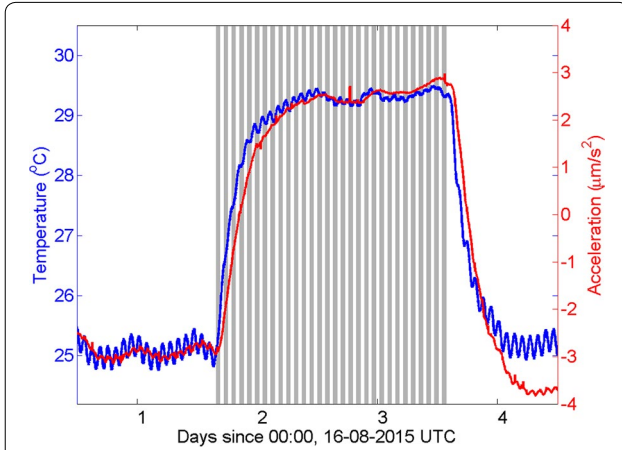
Fig. 7 Acceleration response to heater-induced temperature changes. The step-corrected accelerations show a high correlation to temperature and a delayed response to changes in temperature. The measurements were taken during a thermal test in August 2015 on Swarm C. Gray areas indicate when heaters were active
