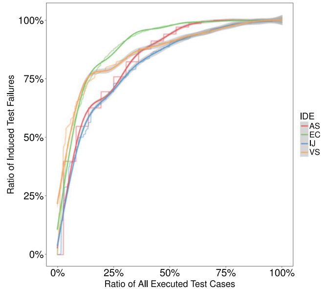
Fig. 11. Accumulated error responsibility of test cases per IDE. Based on 134 projects with \geq 10 run test cases (EC: 112, IJ: 9, AS: 1, VS 12).
