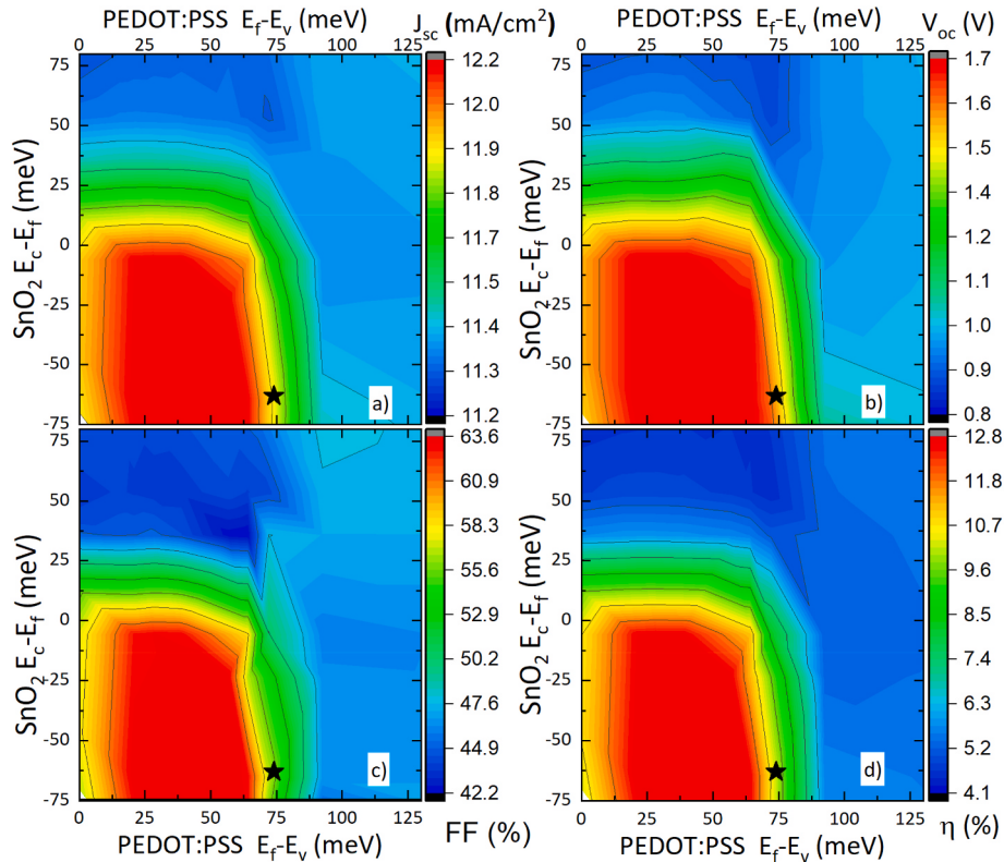
Fig. 5. Contour plot of the simulated external parameters of the 2T tandem solar cells: (a) J_{sc} , (b) V_{oc} , (c) FF and (d) \eta as a function of energy alignment in SnO 2 ( E_c - E_f ) and PEDOT:PSS ( E_f - E_v ). Note that star symbol indicates the energy alignment of the baseline tandem device.
